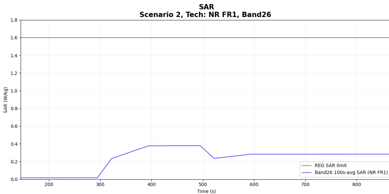
Figure 7-14 Time-averaged SAR
