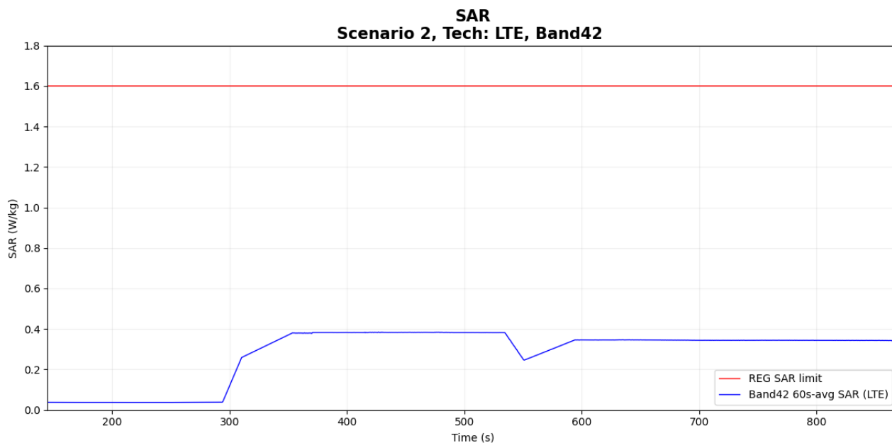
Figure 7-12 Time-averaged SAR
