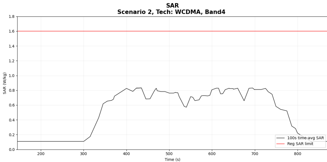
Figure 6- 12 Time-averaged SAR
