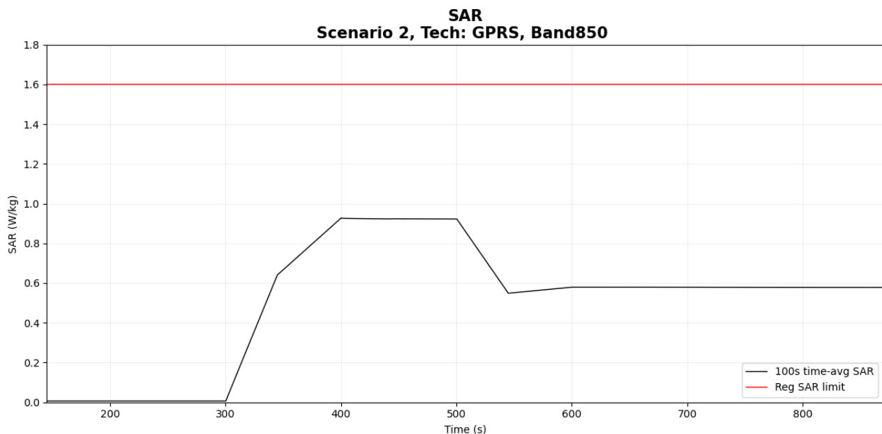
Figure 6- 5 Time-averaged SAR
