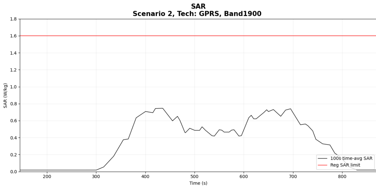
Figure 6- 8 Time-averaged SAR
