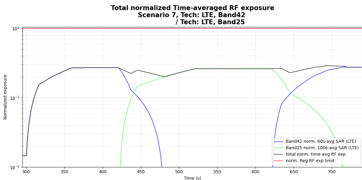
Figure 6- 24 Normalized time-averaged SAR
