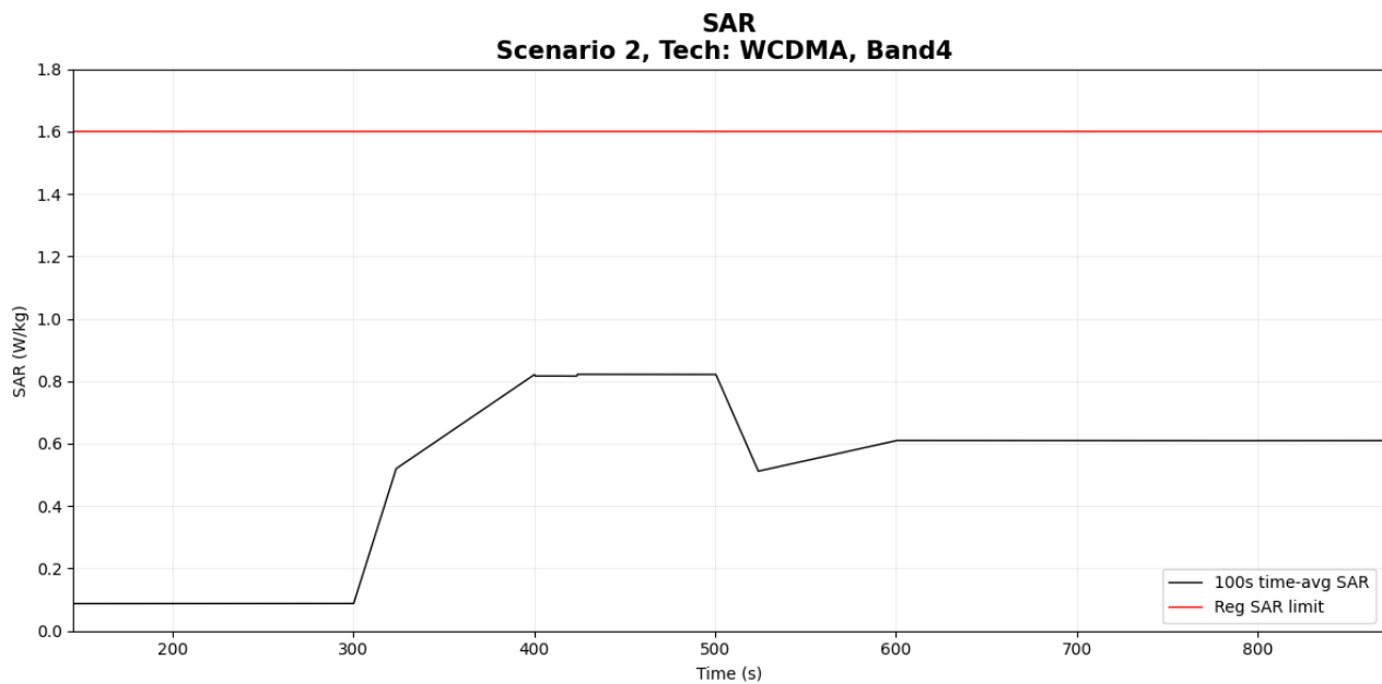
Figure 6- 11 Time-averaged SAR
