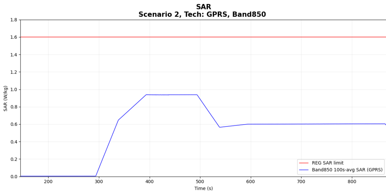
Figure 7-2 Time-averaged SAR
