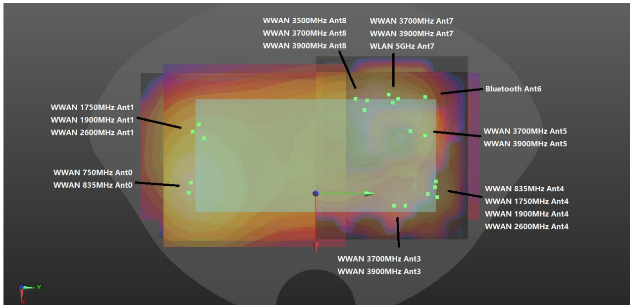
Hotspot WWAN+WLAN+BT Back 5mm
