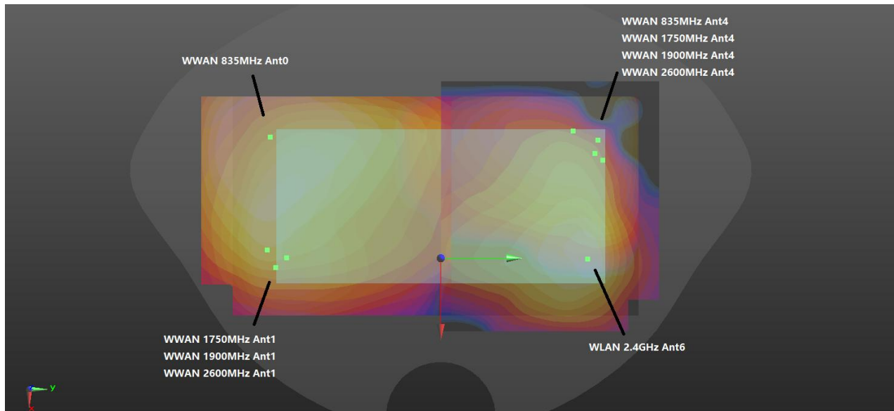
Body worn WWAN+WLAN Front 13mm
