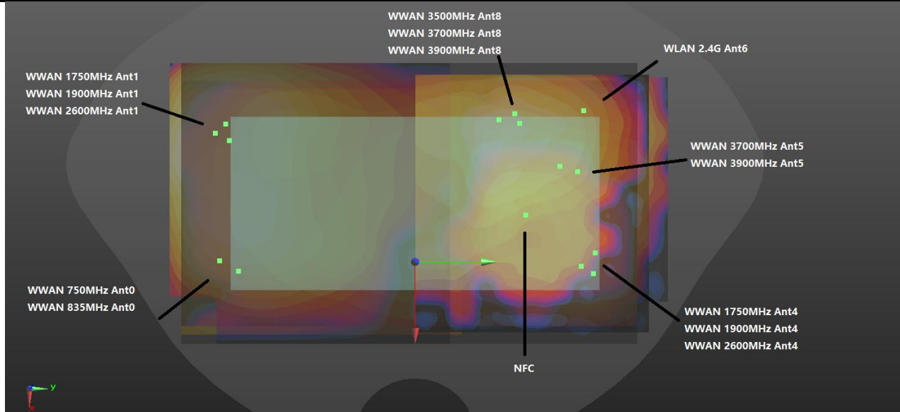
Extremity WWAN+WLAN+NFC Back 0mm
