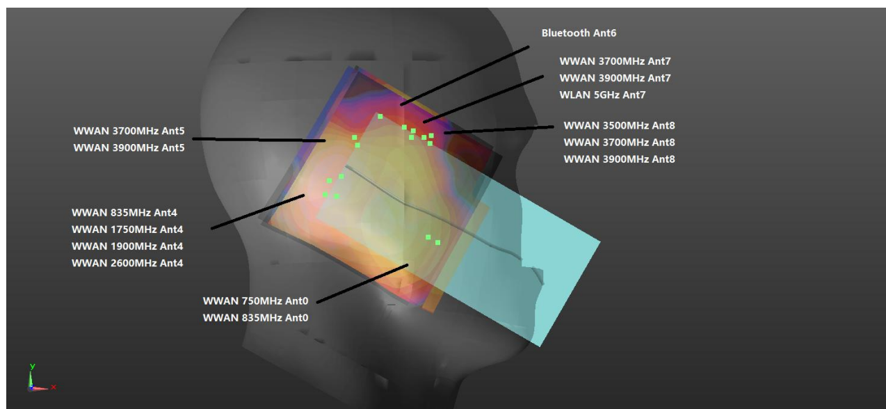
Head WWAN+WLAN+BT Left Cheek 0mm
