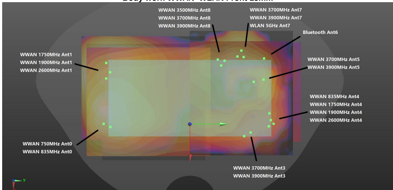
Body worn WWAN+WLAN+BT Back 5mm
