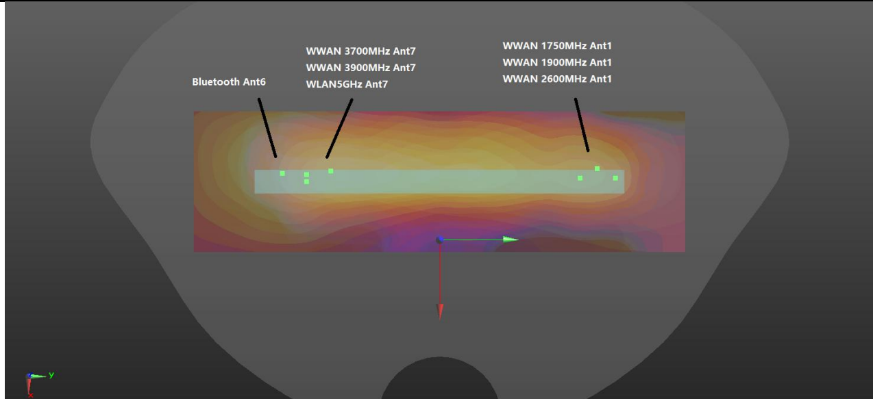
Hotspot WWAN+WLAN+BT Right Side 5mm
