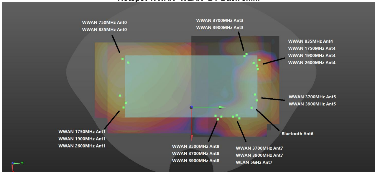
Hotspot WWAN+WLAN+BT Front 5mm
