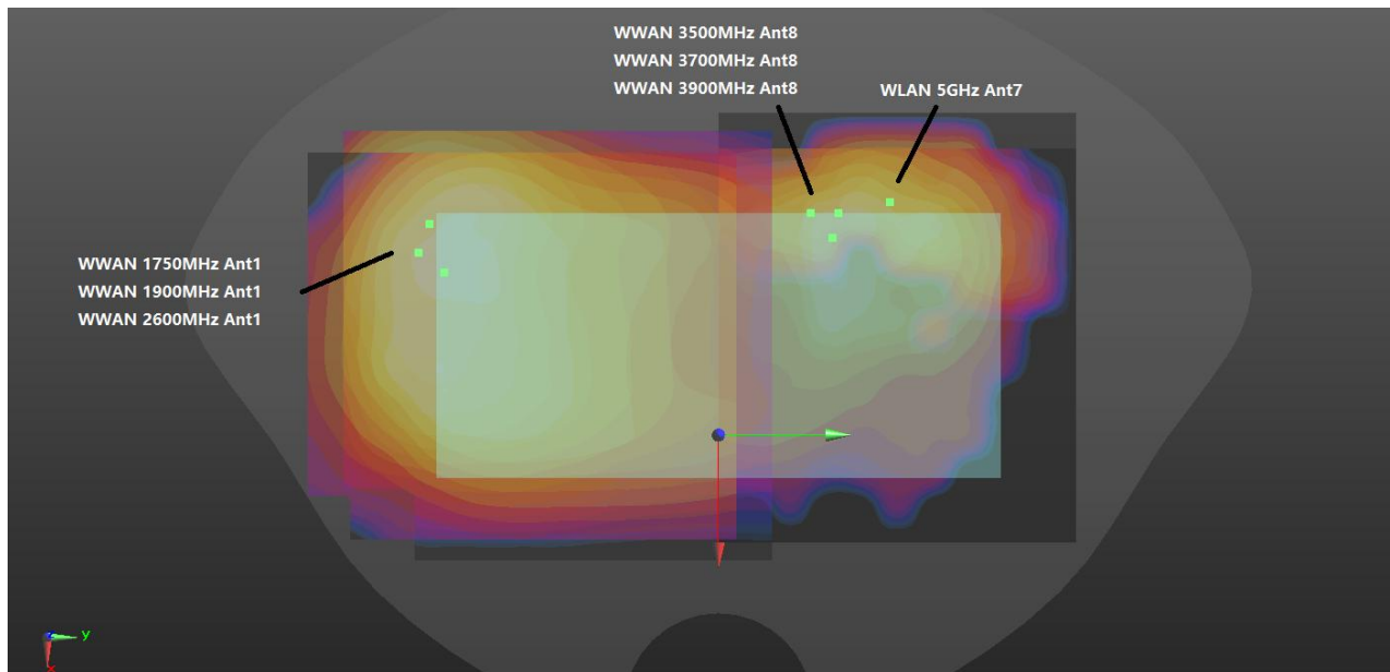
Body worn WWAN+WLAN Back 19mm
