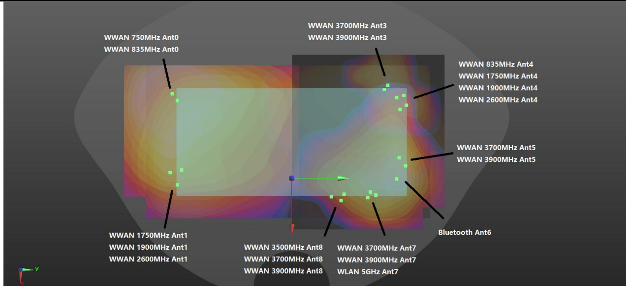
Body worn WWAN+WLAN+BT Front 5mm
