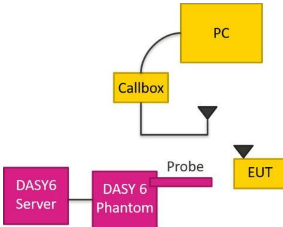
Figure 7-1 TA-SAR wireless test environment
