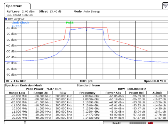
Plot on Channel 7115MHz
