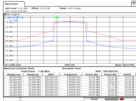
Plot on Channel 6885MHz
