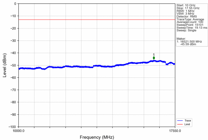
Band4_RMC_MCH_1732.6MHz_12.2kbps RMC_NTNV
