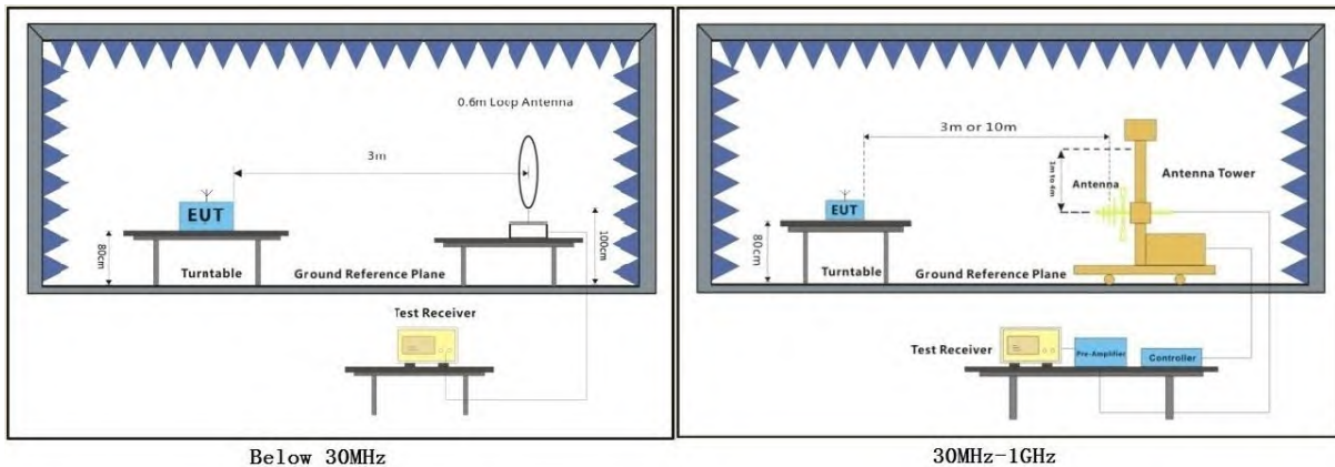
Below 30MHz
