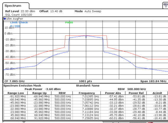
Plot on Channel 7085MHz
