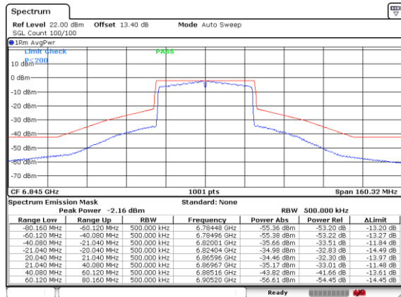
Plot on Channel 6845MHz
