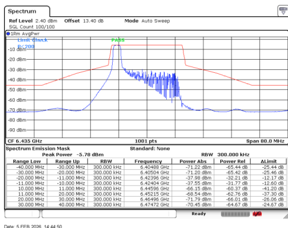
Plot on Channel 6435MHz 26RU0
