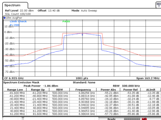
Plot on Channel 6925MHz
