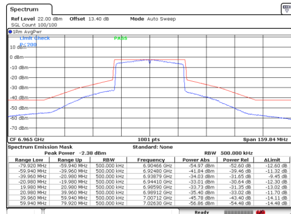
Plot on Channel 6965MHz
