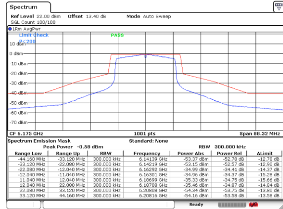
Plot on Channel 6175MHz
