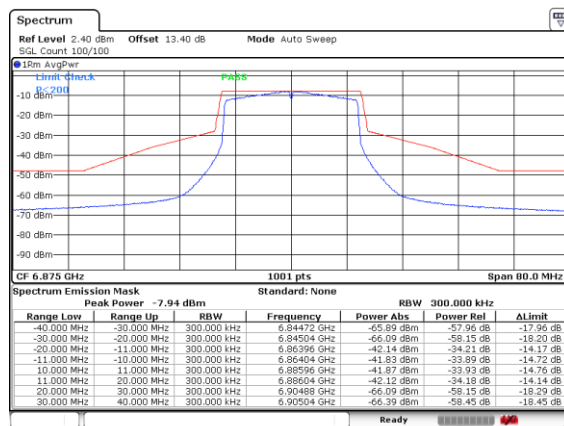
Plot on Channel 6875MHz
