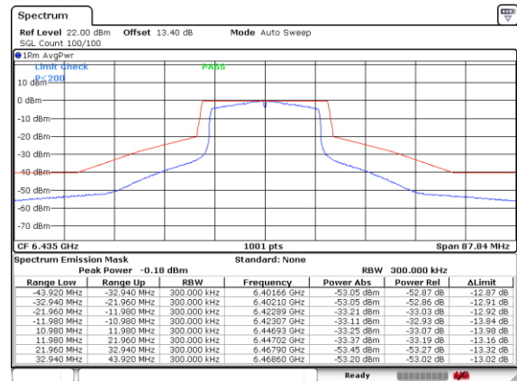
Plot on Channel 6435MHz
