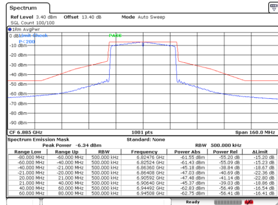
Plot on Channel 6885MHz
