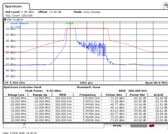
Plot on Channel 5955MHz 52RU37
