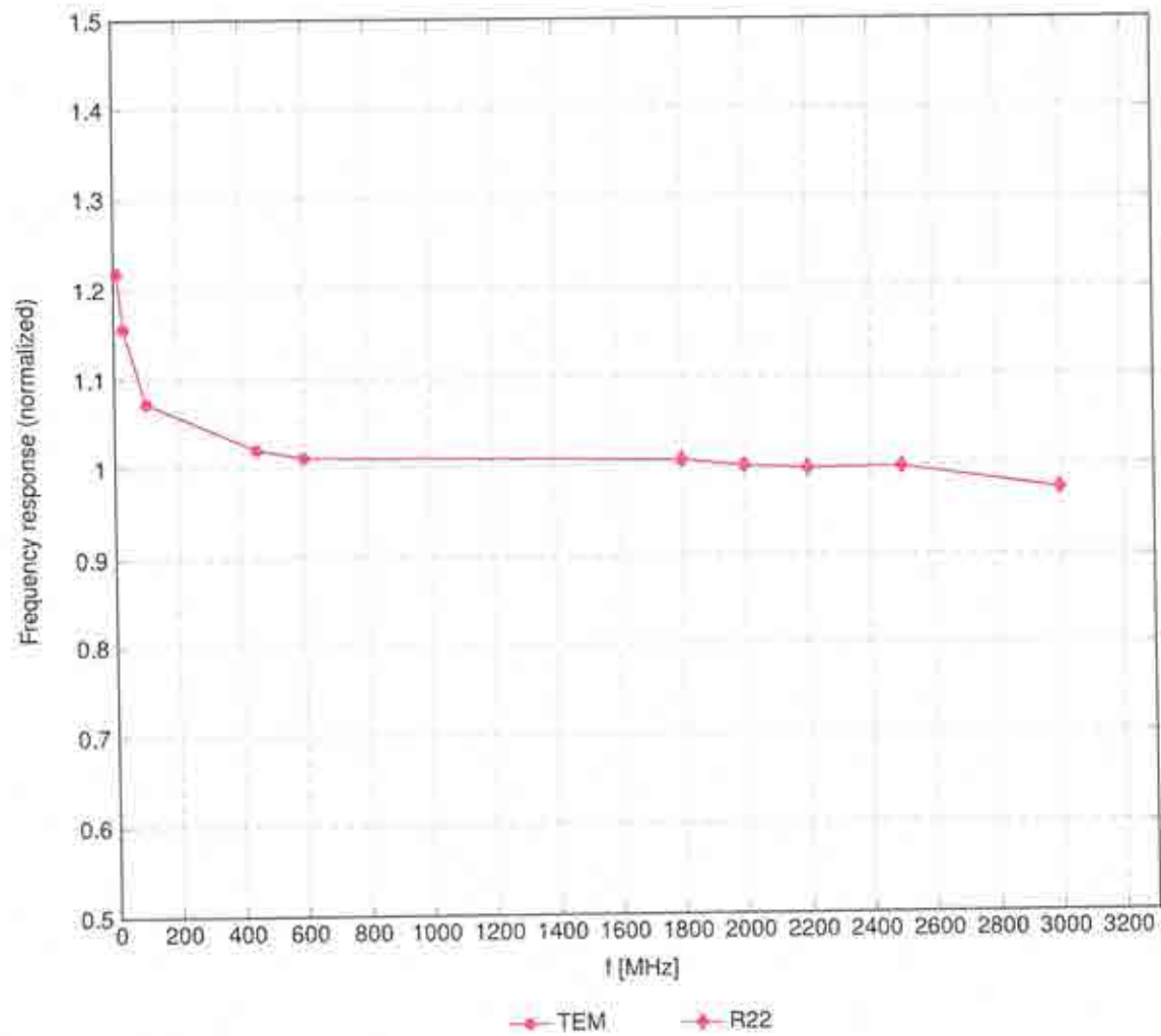
Frequency Response of E-Field (TEM-Cell:ifi110 EXX, Waveguide:R22)
