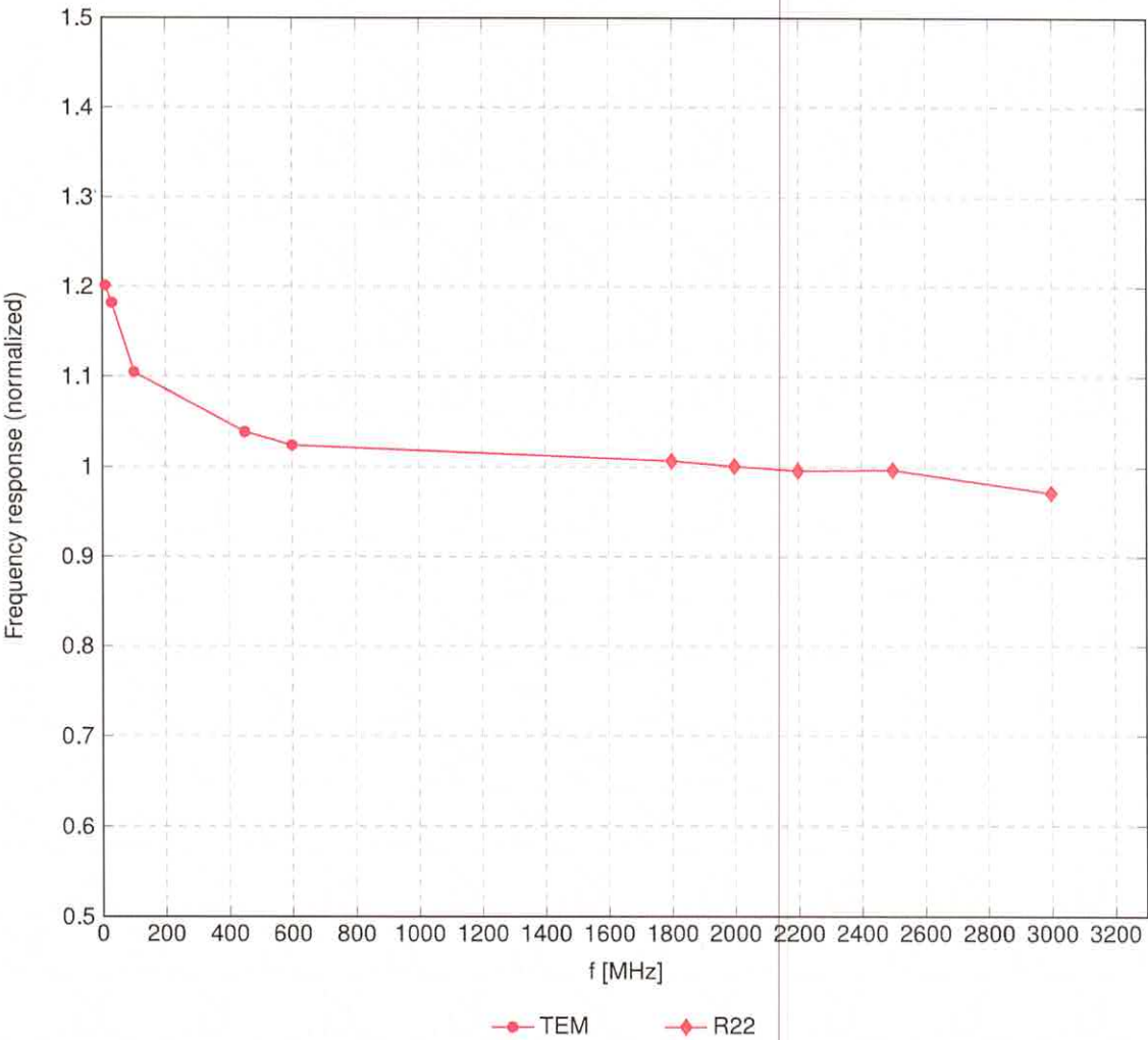
Frequency Response of E-Field (TEM-Cell:ifi1110 EXX, Waveguide:R22)
