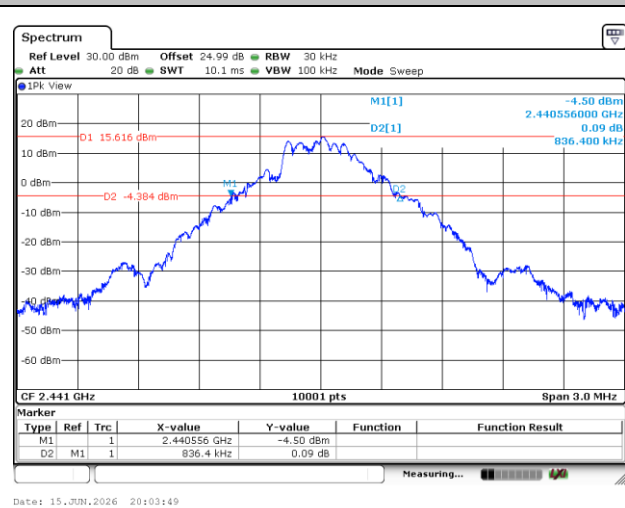
20 dB Bandwidth Plot in Channel 39
