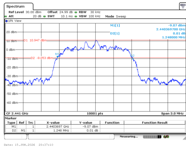
20 dB Bandwidth Plot in Channel 39
