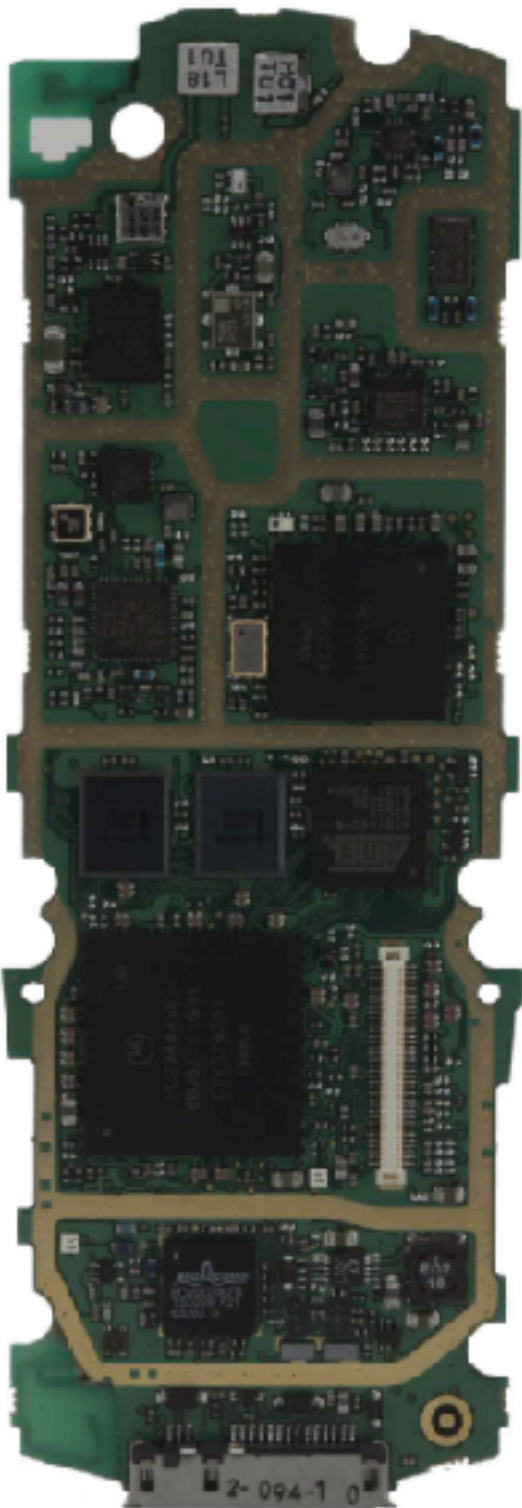
Front View (Shields Removed)
