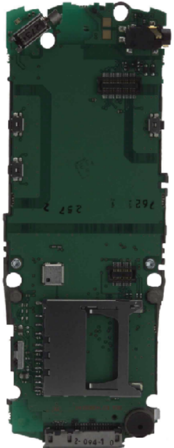
Front View Daughter Board with Shields
