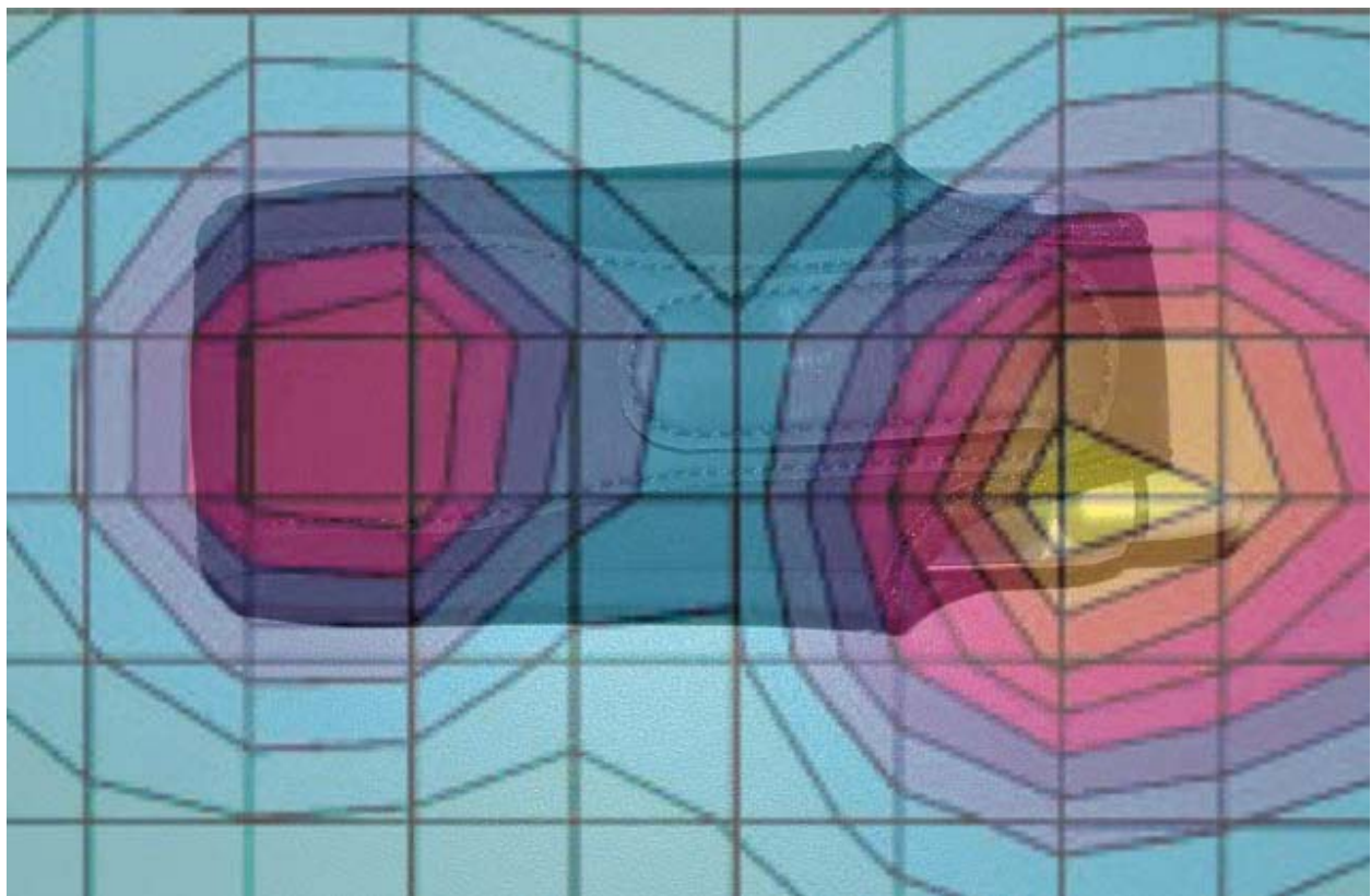
Figure 2. Typical 1900 MHz Body-Worn Contour Overlaid on Phone using #MOTPQ0433K
