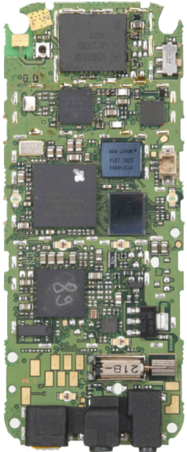
Rear View (Shields Removed)
