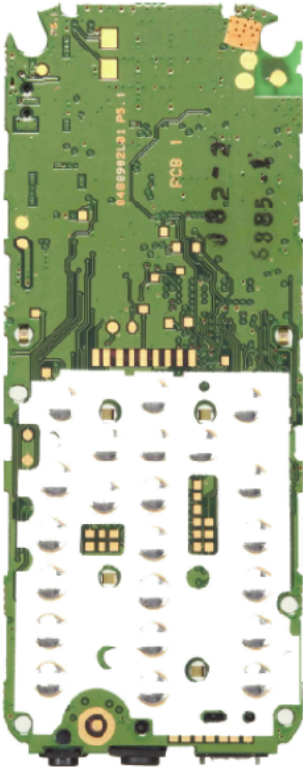
Front View (Shields Removed)
