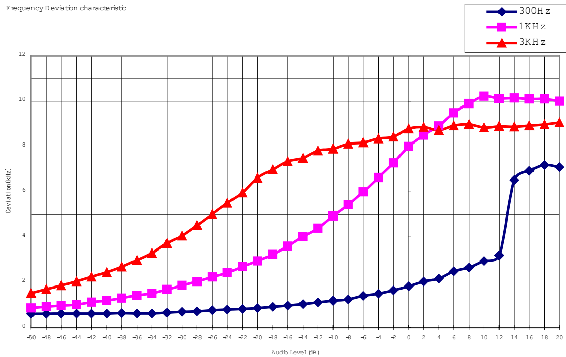
Frequency Deviation characteristic
