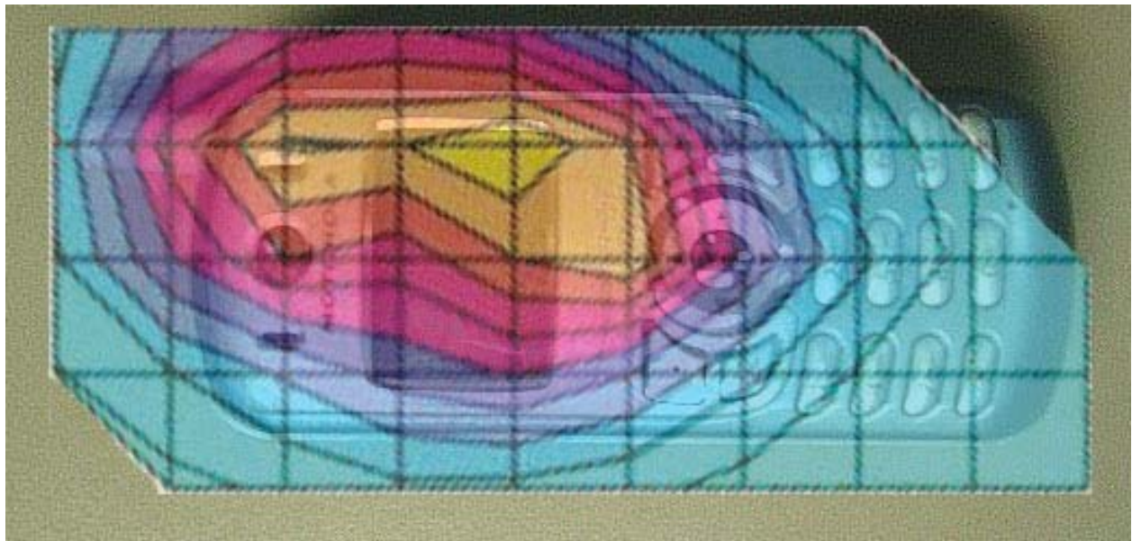
Figure 1. Typical 800MHz Head Adjacent Contour Overlaid on Phone (Cheek Touch)
