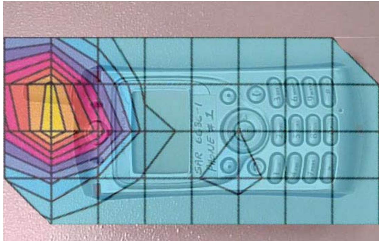
Figure 4. Typical 1900MHz Contour Overlaid on Phone (15 ° Tilt)
