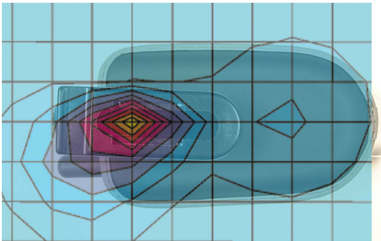
Figure 2. Typical 1900 MHz Body-Worn Contour Overlaid on Phone
