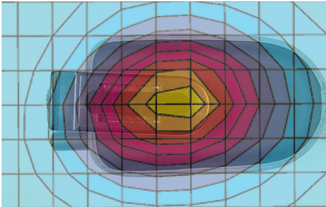
Figure 1. Typical 800 MHz Body-Worn Contour Overlaid on Phone
