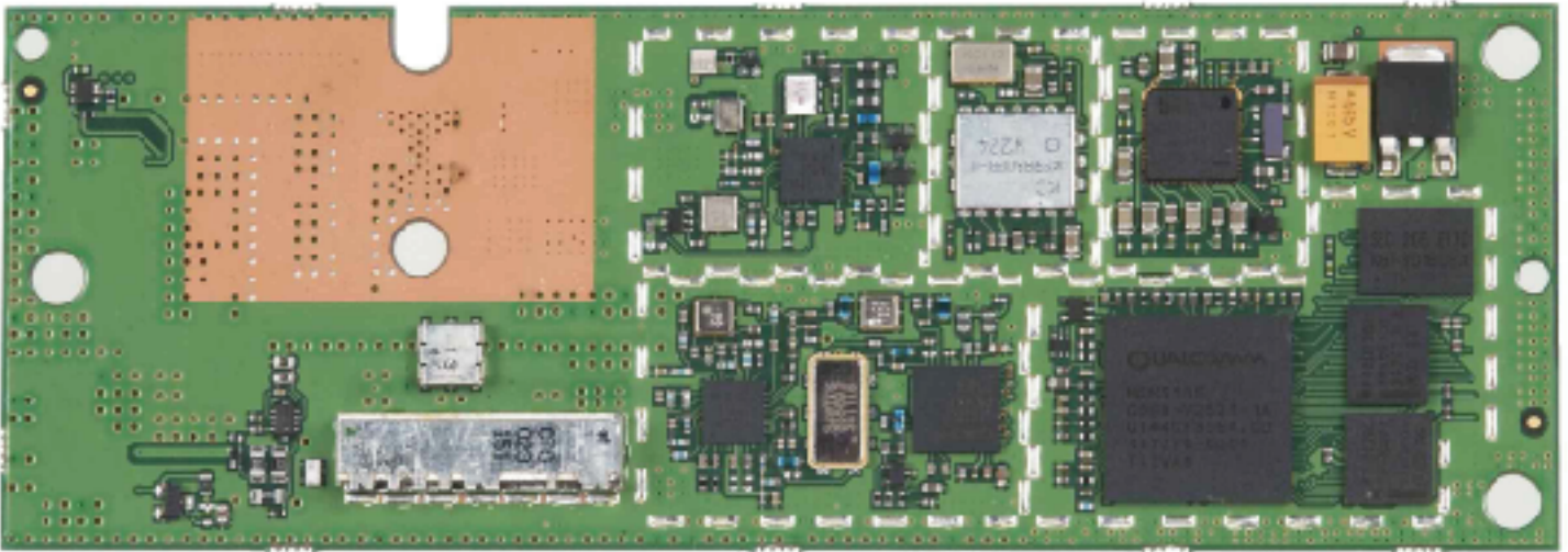
NAB Board (Top View)
