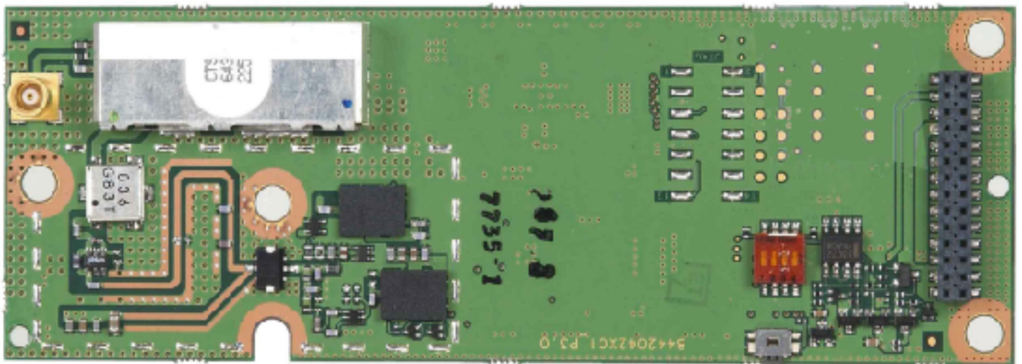
NAB Board (Bottom View)
