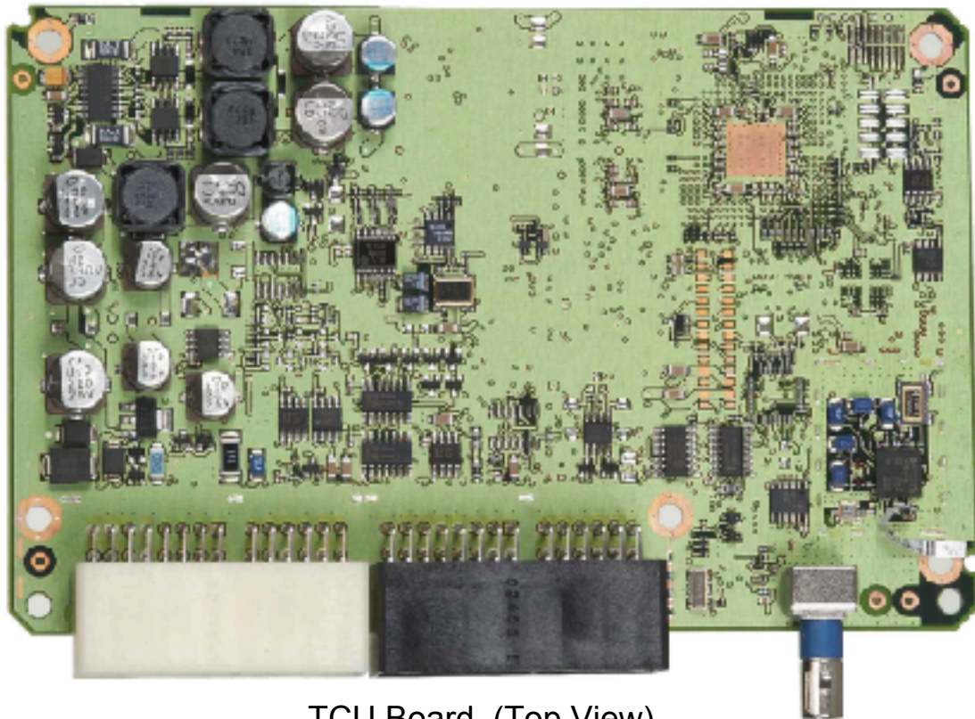
TCU Board (Top View)
