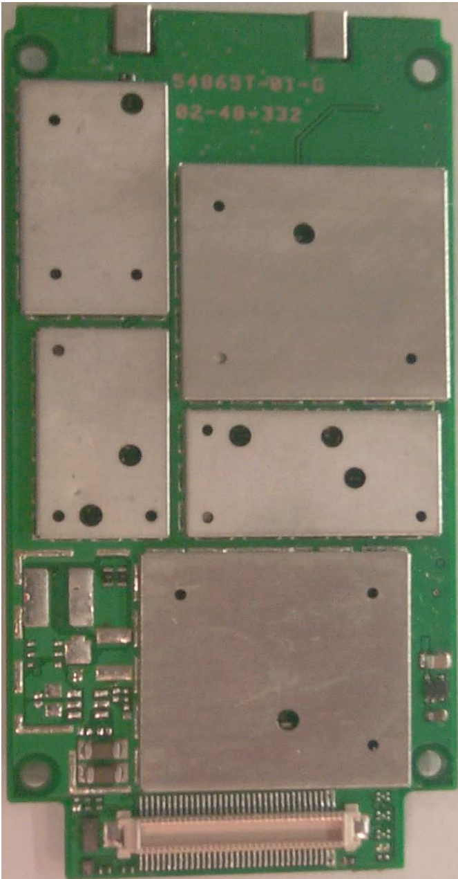
Front View (With Shield)
