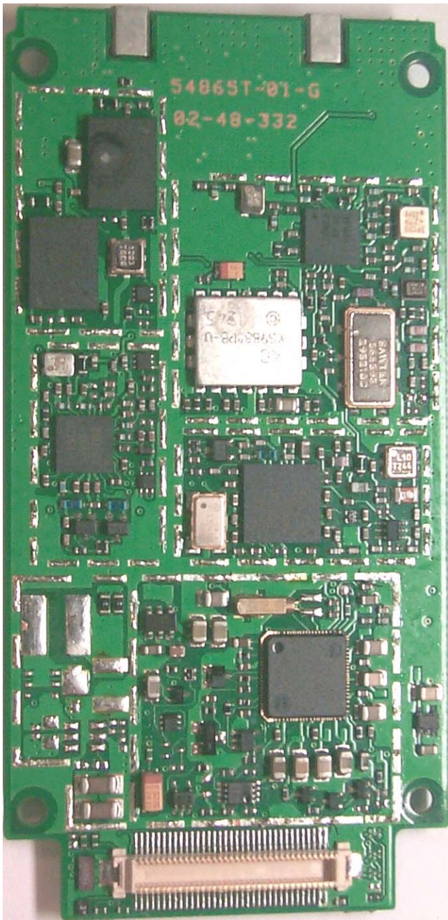
Front View (Shields Removed)
