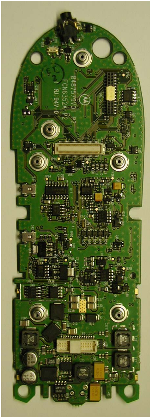
Rear View (Shields Removed)
