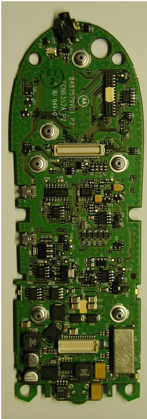
Rear View (With Shield)
