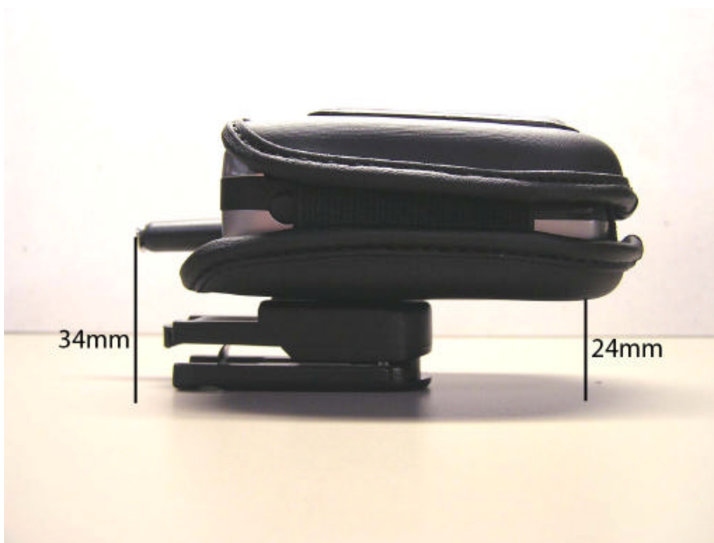
Figure 16. Side of Phone, in Case, with Antenna Retracted
