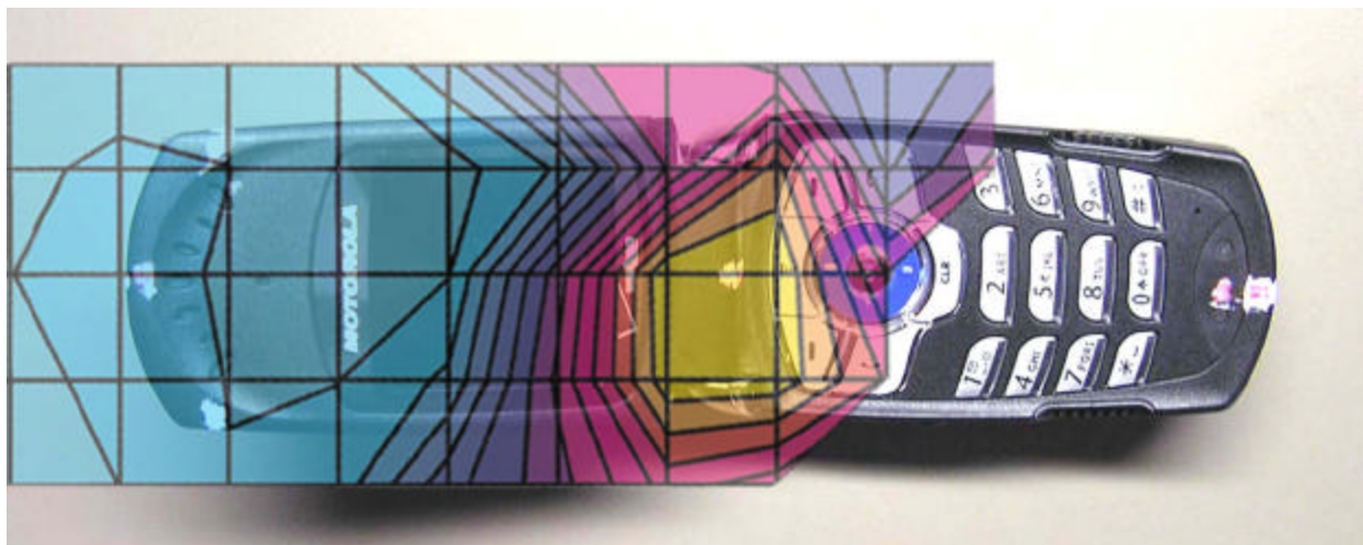
Figure 1. Typical 1900MHz Head Adjacent Contour Overlaid on Phone with Antenna Extended (Cheek Touch)
