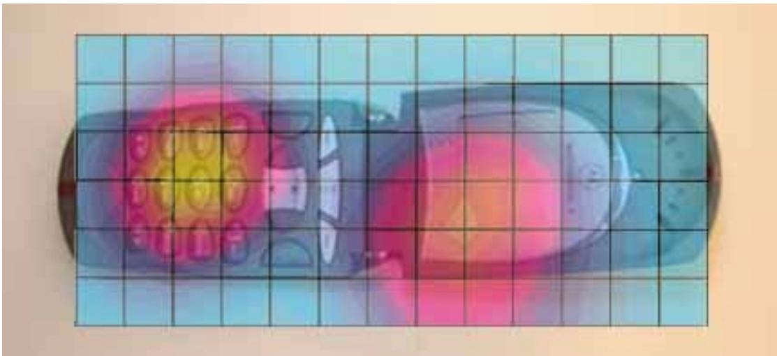
Figure 10. Typical 1900 MHz PTT Contour Overlaid on Phone with Antenna Fixed (Flip Open)
