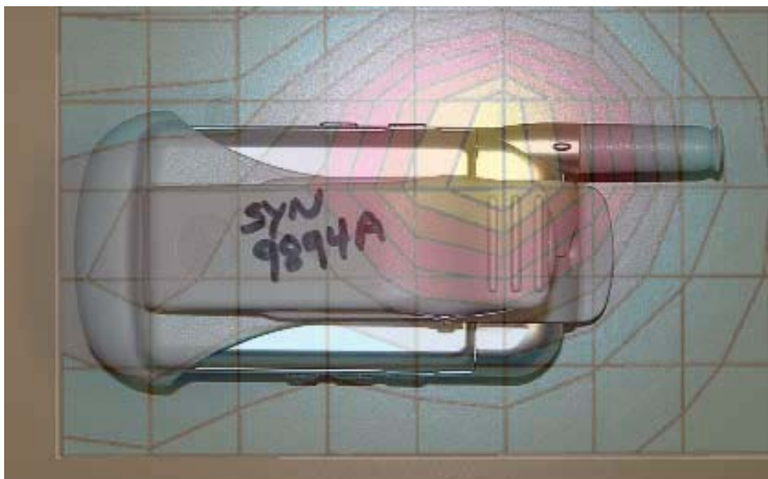
Figure 11. Typical 1900 MHz Body-Worn Contour Overlaid on Phone with Antenna Retracted
