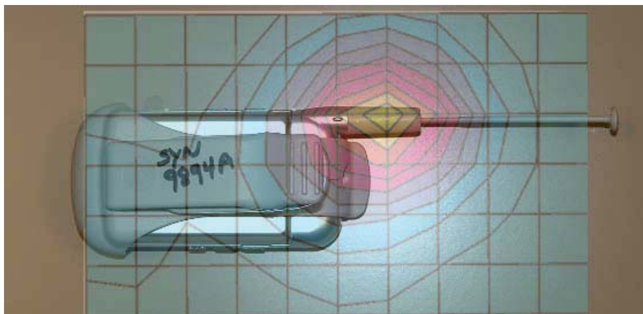
Figure 12. Typical 1900 MHz Body-Worn Contour Overlaid on Phone with Antenna Extended
