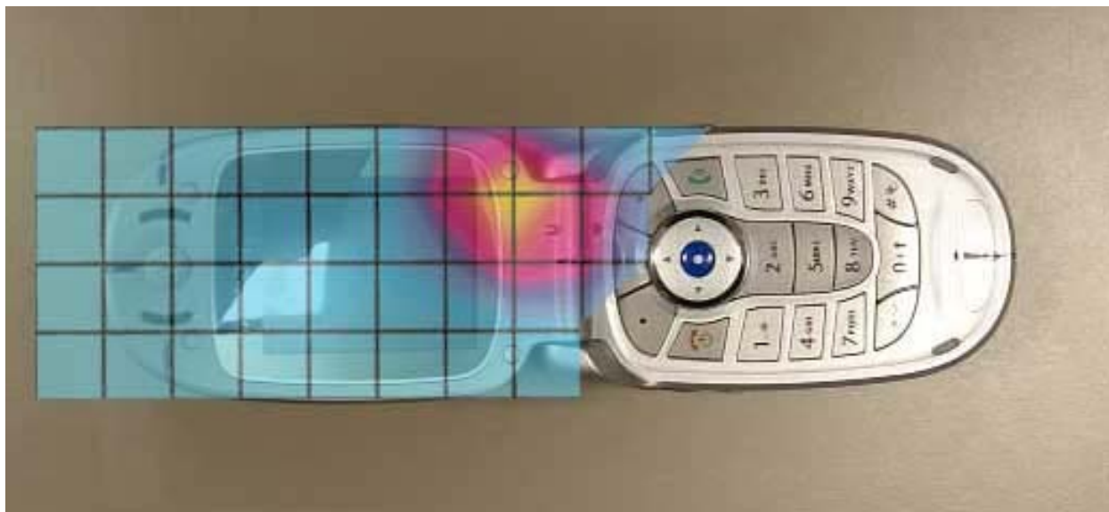
Figure 3. Typical 1900MHz Right Head Adjacent Contour Overlaid on Phone with Antenna Fixed (Cheek Touch)
