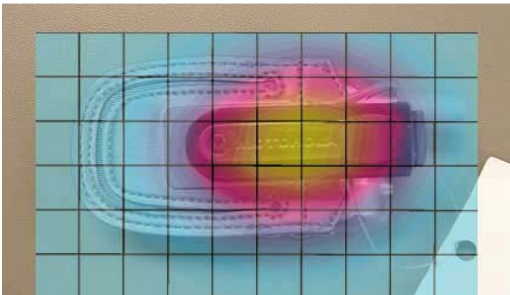
Figure 7. Typical 850 MHz Body-Worn Contour Overlaid on Phone with Antenna Fixed (Half Silver Pouch)
