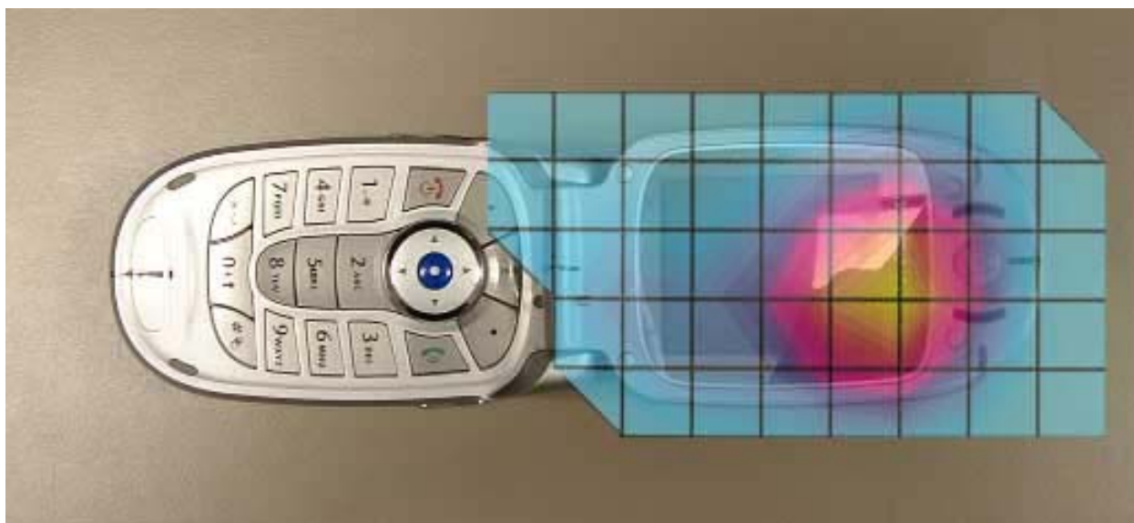
Figure 4. Typical 1900MHz Right Head Adjacent Contour Overlaid on Phone with Antenna Fixed (15° Tilt)
