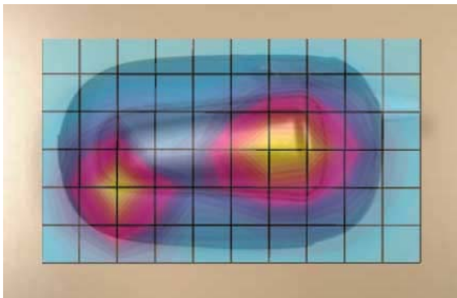
Figure 6. Typical 1900 MHz Body-Worn Contour Overlaid on Phone with Antenna Fixed (Mercury Eva Pouch)
