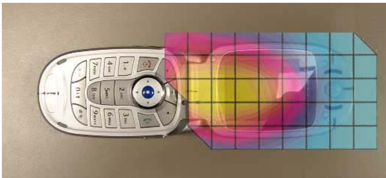
Figure 2. Typical 850MHz Left Head Adjacent Contour Overlaid on Phone with Antenna Fixed (15° Tilt)
