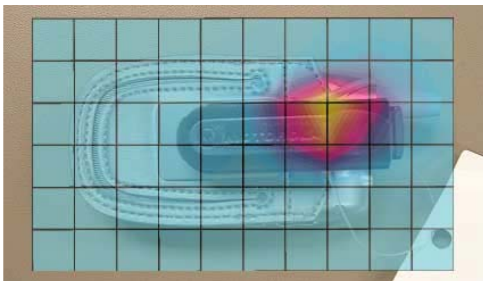
Figure 8. Typical 1900 MHz Body-Worn Contour Overlaid on Phone with Antenna Fixed (Half Silver Pouch)
