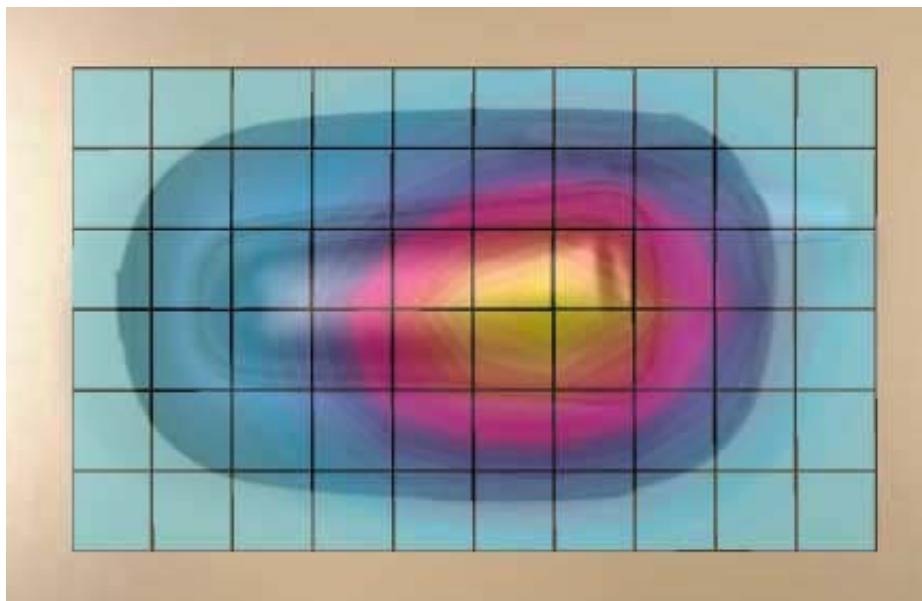
Figure 5. Typical 850 MHz Body-Worn Contour Overlaid on Phone with Antenna Fixed (Mercury Eva Pouch)
