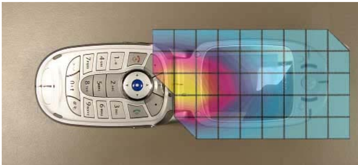
Figure 1. Typical 850MHz Left Head Adjacent Contour Overlaid on Phone with Antenna Fixed (Cheek Touch)
