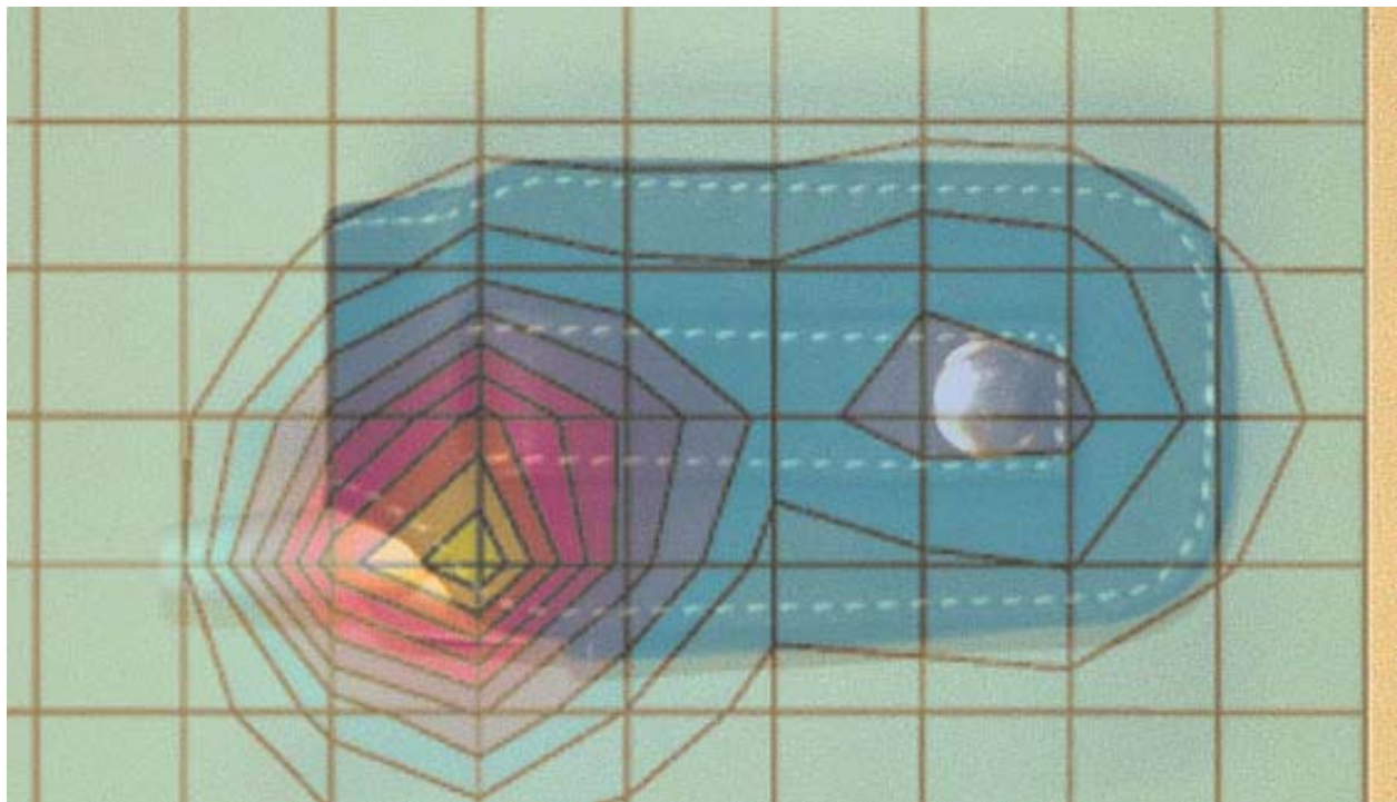
Figure 2. Typical 1900 MHz Body-Worn Contour Overlaid on Phone
