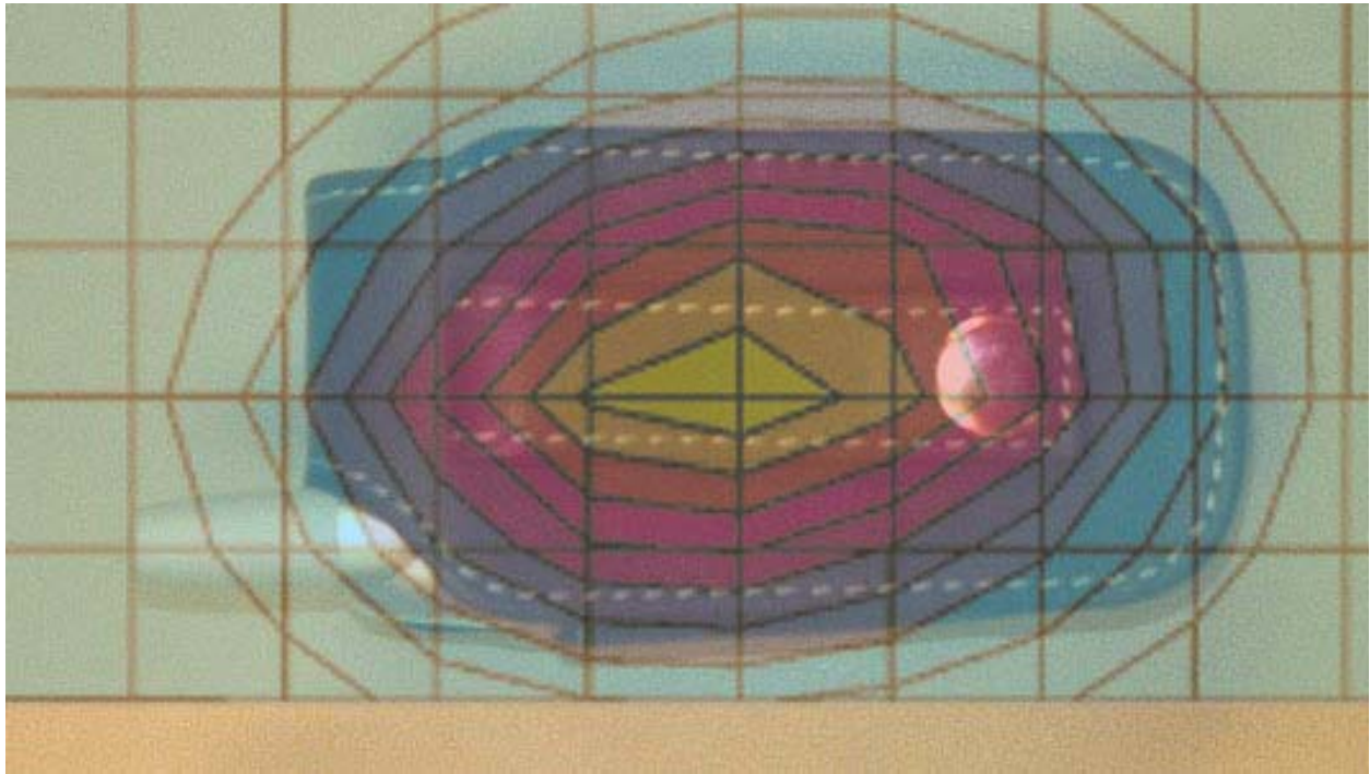
Figure 1. Typical 800 MHz Body-Worn Contour Overlaid on Phone
