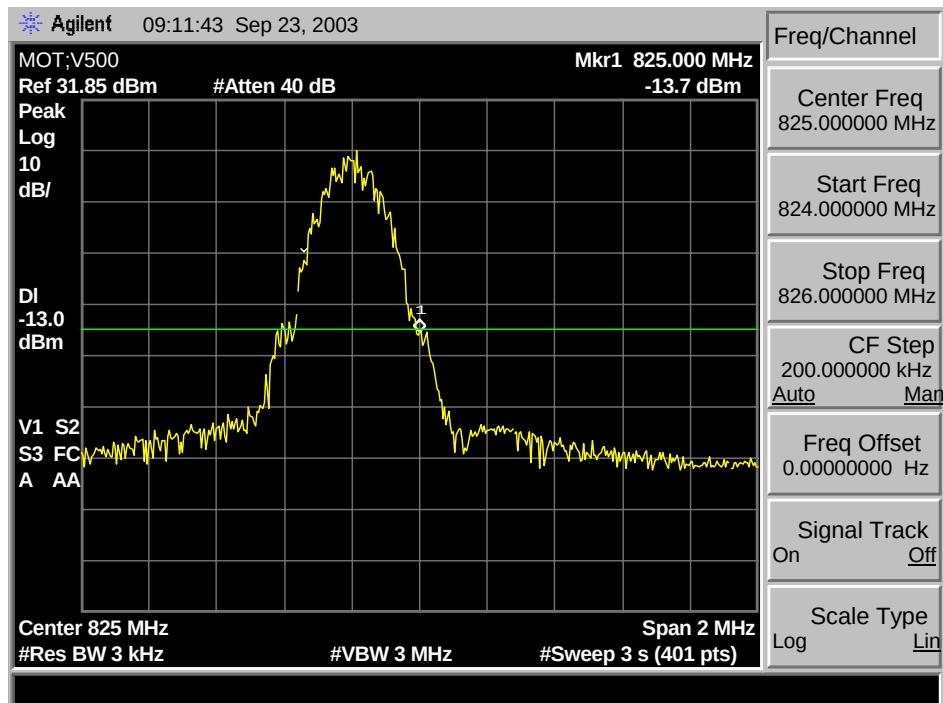
GSM 850 A*(Lower) Max Block Edge
