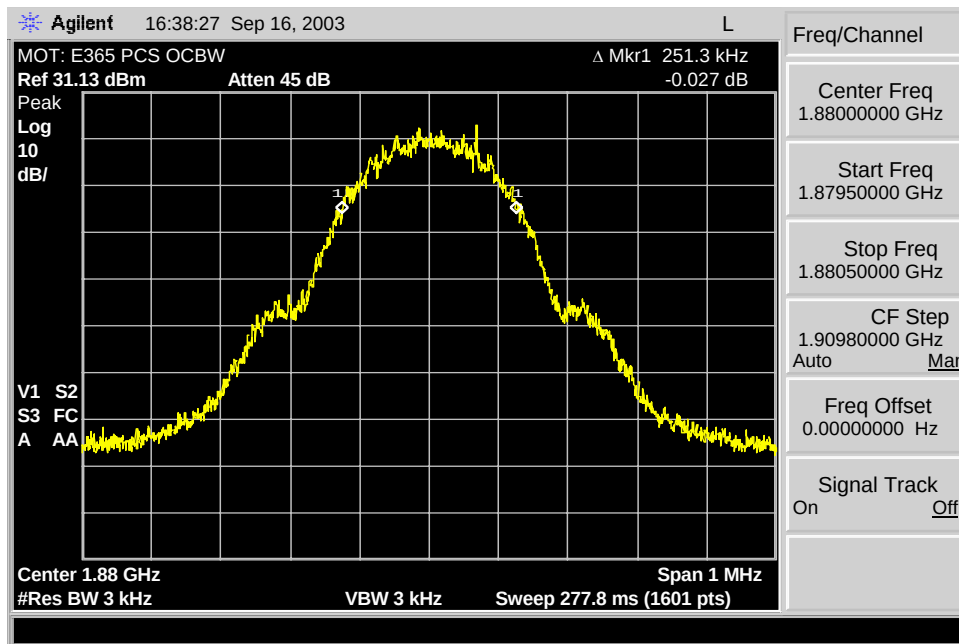
1900 GSM Occupied Band
