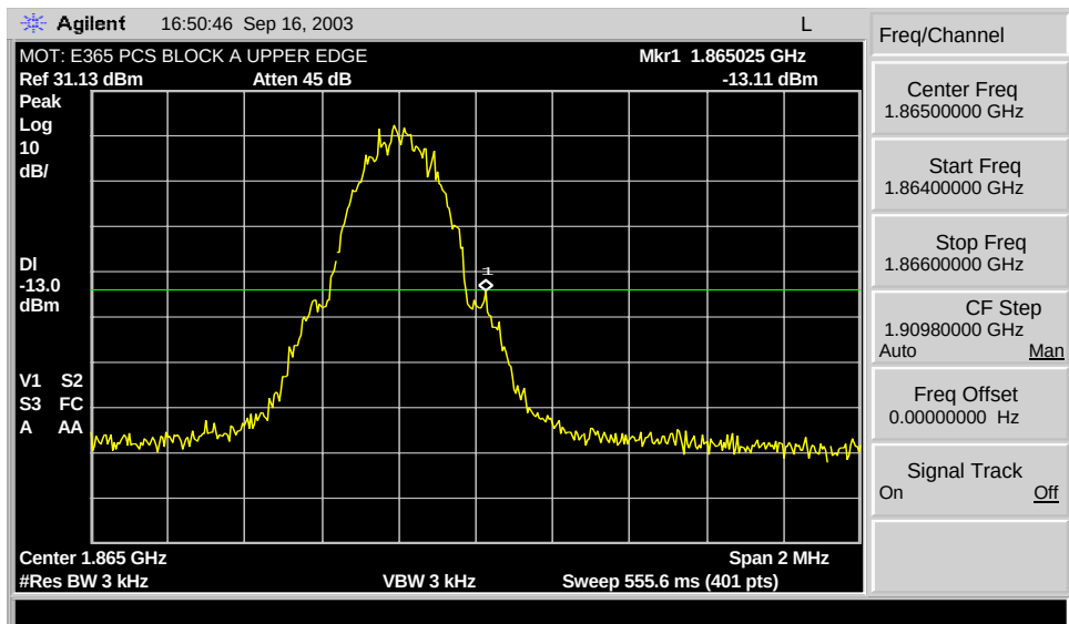
GSM 1900 A Max. Block Edge
