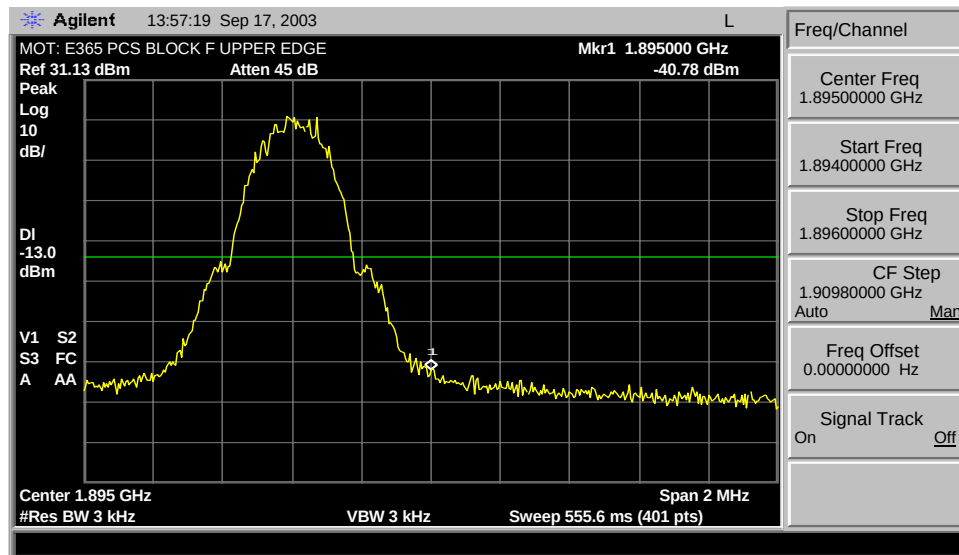
GSM 1900 F Max. Block Edge
