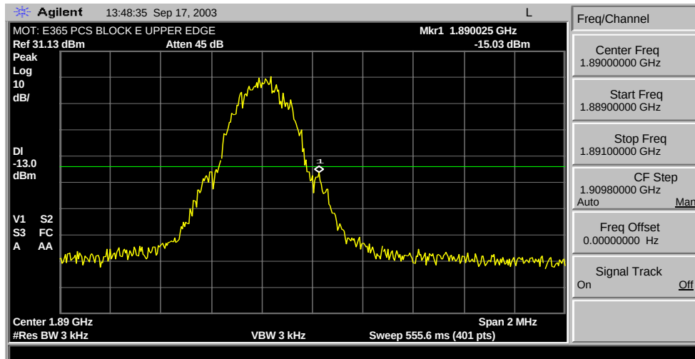
GSM 1900 E Max. Block Edge
