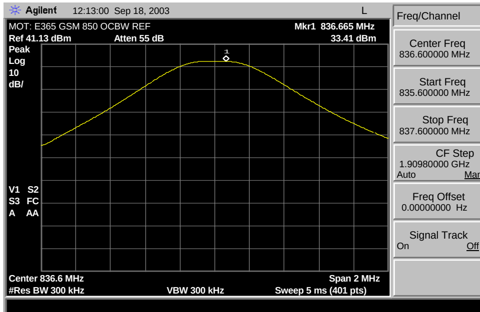
850 GSM Reference Plot
