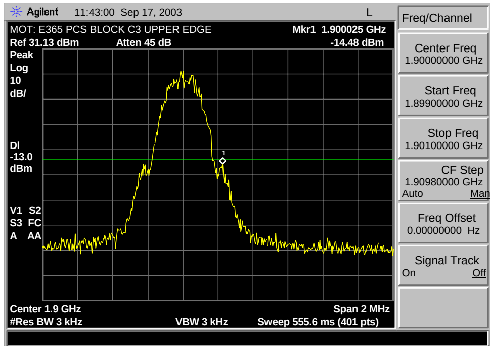
GSM 1900 C3 Max Block Edge
