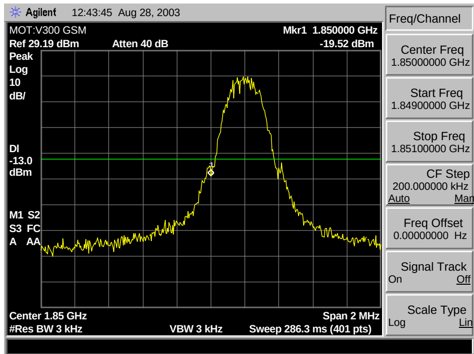
GSM 1900 Lower Band Edge
