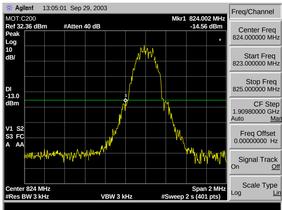
GSM 850 Lower Band Edge
