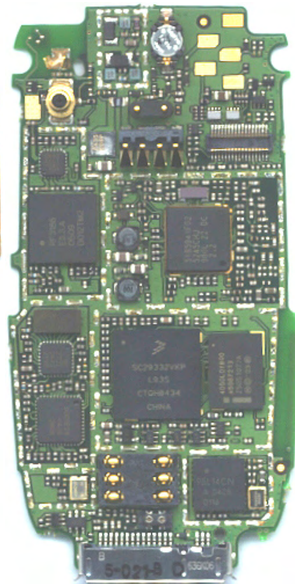
Main Board (shields off)
