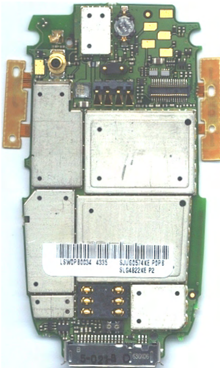
Main Board (shields on)
