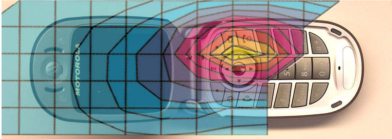
Figure 1. Typical 800MHz Head Adjacent Contour Overlaid on Phone (Cheek Touch)
