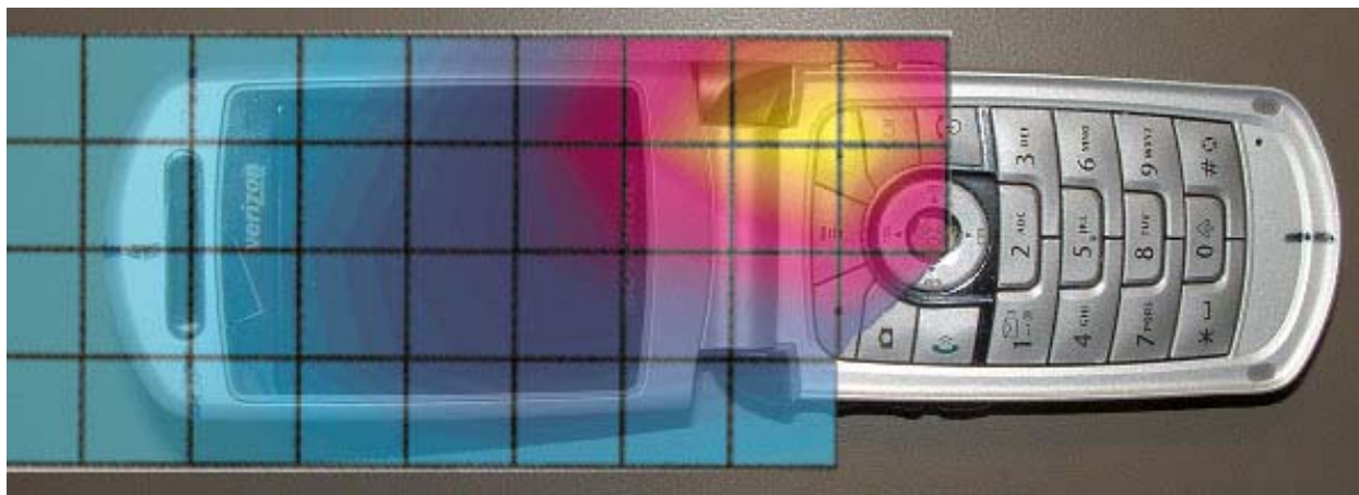
Figure 3. Typical 800MHz Head Adjacent Contour Overlaid on Phone with Antenna Retracted (Cheek Touch)
