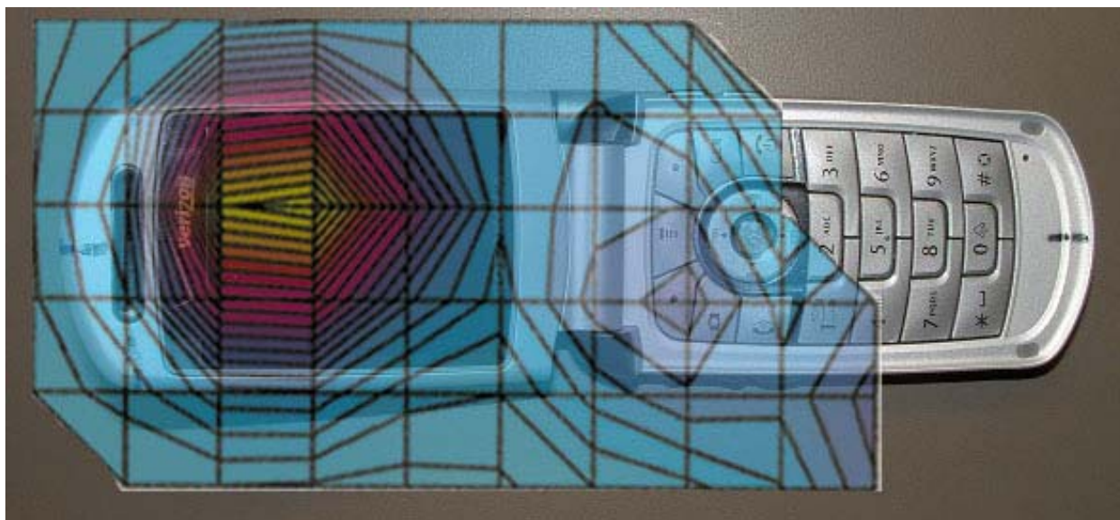
Figure 8. Typical 1900MHz Head Adjacent Contour Overlaid on Phone with Antenna Retracted (15 ° Tilt)
