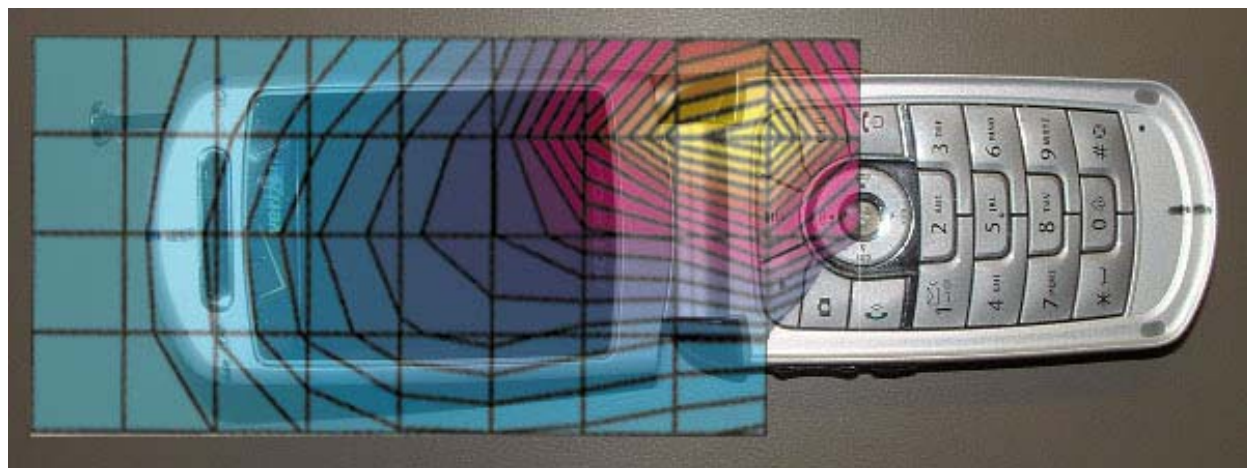
Figure 1. Typical 800MHz Head Adjacent Contour Overlaid on Phone with Antenna Extended (Cheek Touch)
