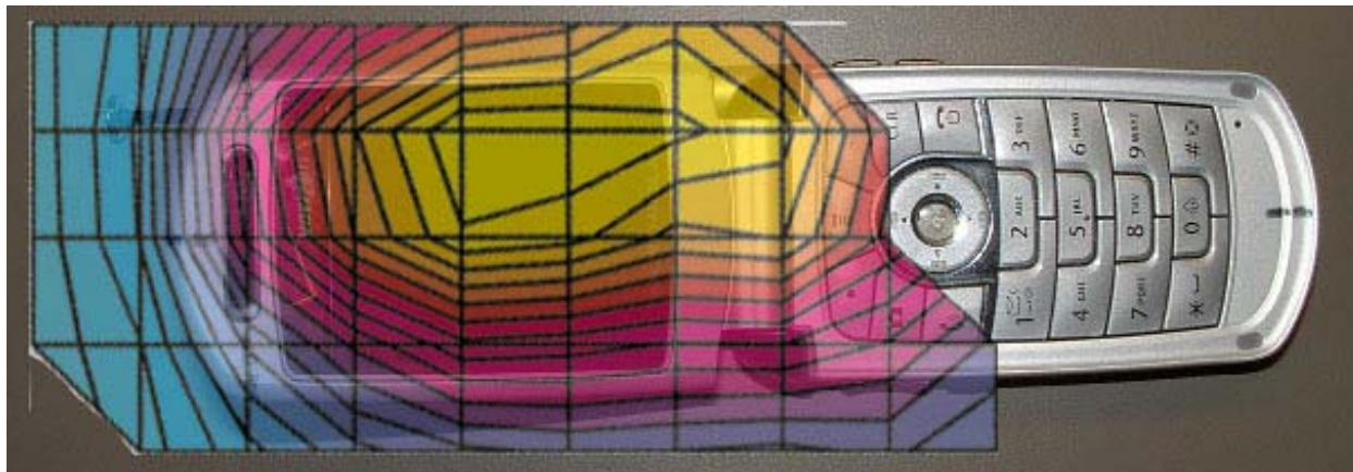
Figure 5. Typical 800MHz Head Adjacent Contour Overlaid on Phone with Antenna Extended (15 ° Tilt)
