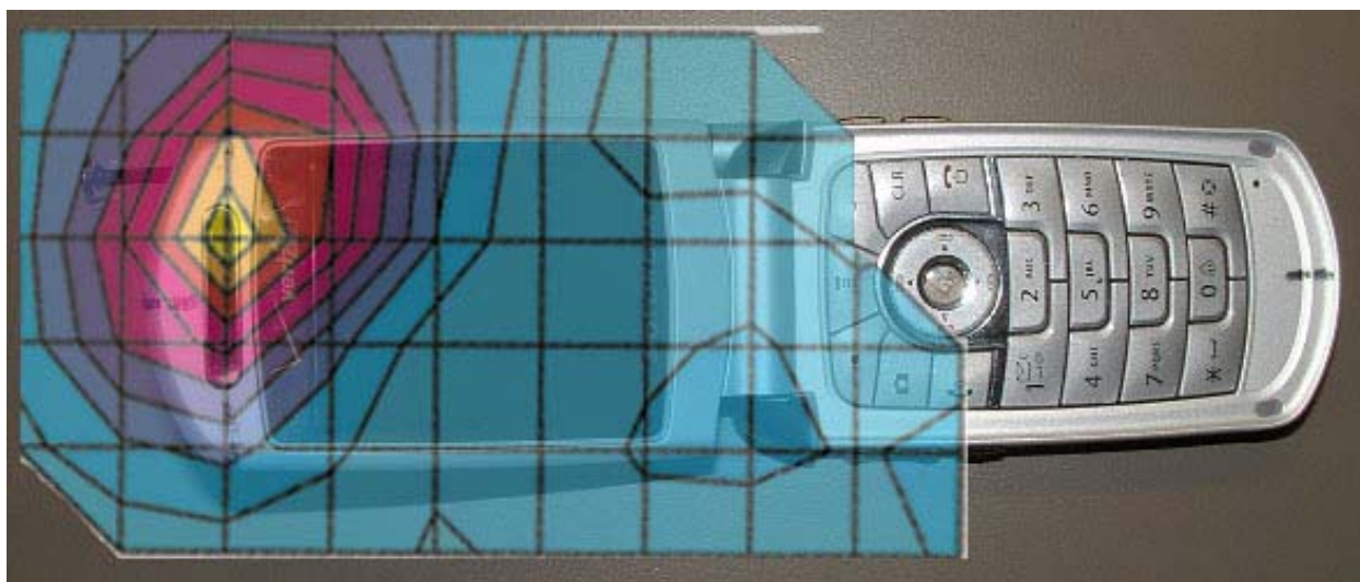
Figure 6. Typical 1900MHz Head Adjacent Contour Overlaid on Phone with Antenna Extended (15 ° Tilt)
