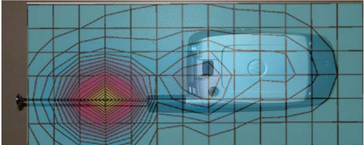
Figure 11. Typical 1900 MHz Body-Worn Contour Overlaid on Phone with Antenna Extended
