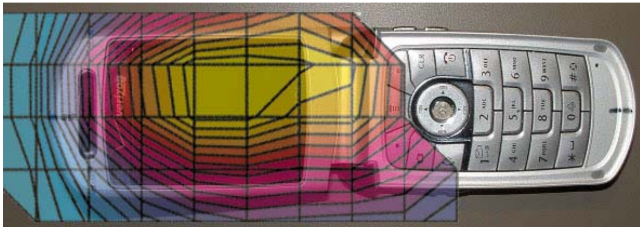
Figure 7. Typical 800MHz Head Adjacent Contour Overlaid on Phone with Antenna Retracted (15 ° Tilt)
