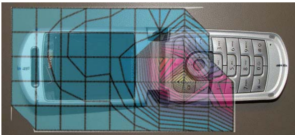
Figure 4. Typical 1900MHz Head Adjacent Contour Overlaid on Phone with Antenna Retracted (Cheek Touch)
