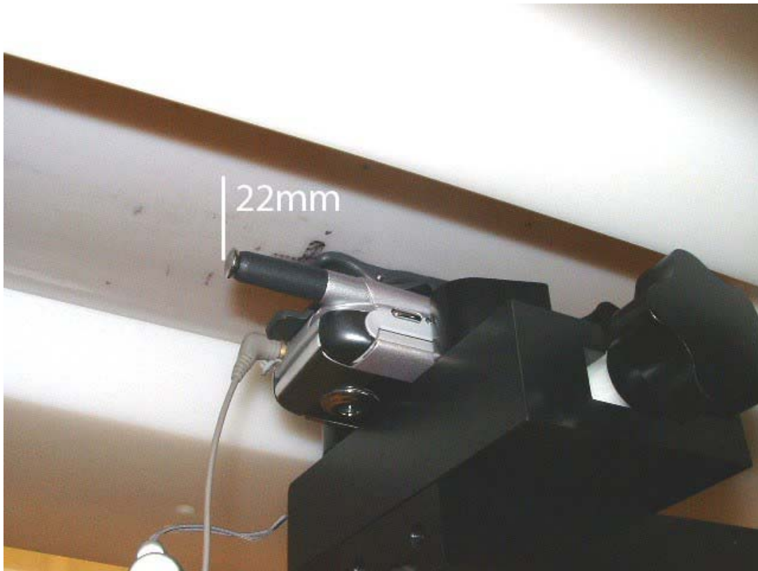
Figure 29. Phone in Holster Against the Flat Phantom with Antenna Retracted
