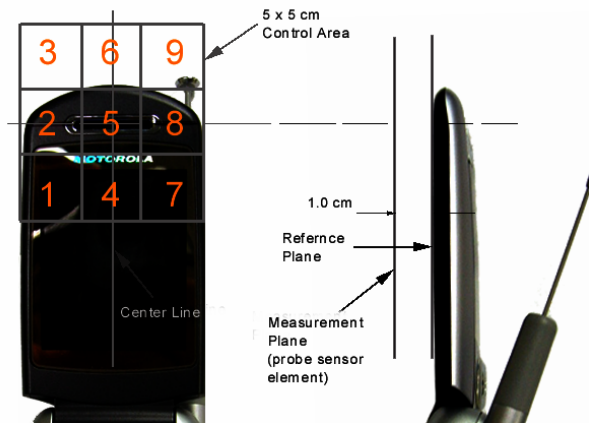
Figure 13 E/H-Field Emissions Test Setup Diagram
