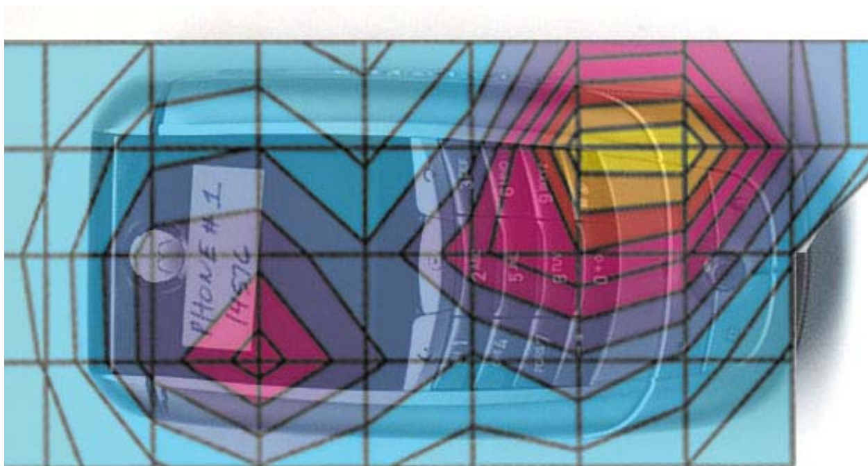
Figure 5. Typical 1900MHz Head Adjacent Contour Overlaid on Phone with Flip Closed (Cheek Touch)
