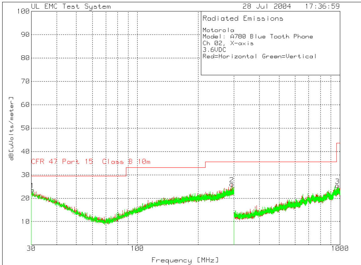
30MHz – 1000MHz Ch. 02 X-Axis
