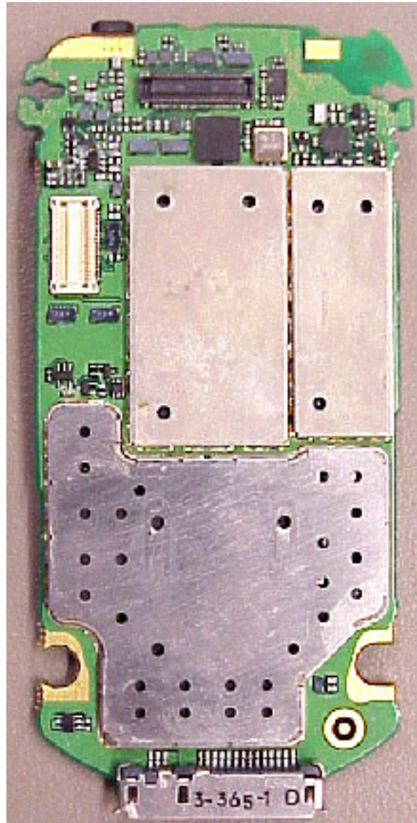
Main Board (shields on)
