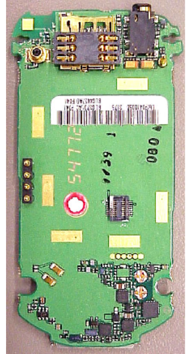
Main Board Rear View
