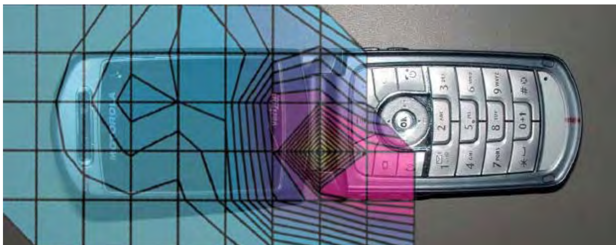
Figure 4. Typical 1900MHz Head Adjacent Contour Overlaid on Phone with Antenna Retracted (Cheek Touch)
