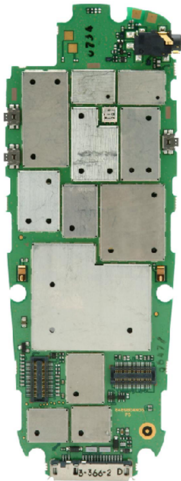
Front View with Shields
