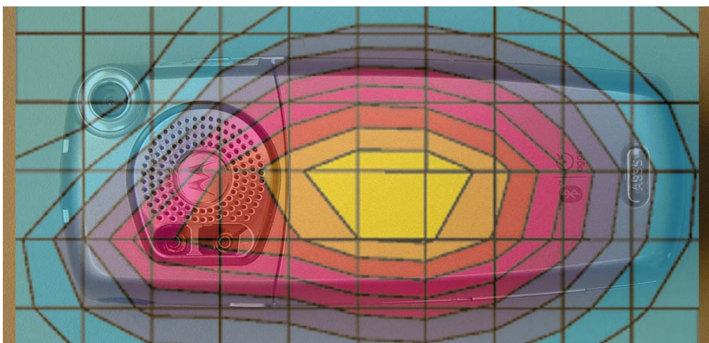
Figure 7. Typical 850MHz GSM Body Worn Contour Overlaid on Phone
