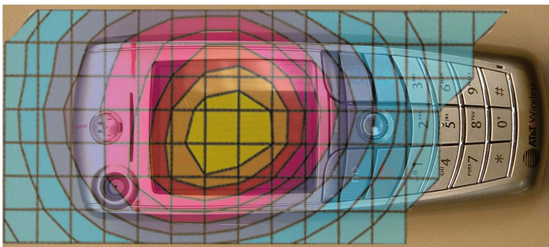
Figure 1. Typical 850MHz GSM Head Adjacent Contour Overlaid on Phone (Cheek Touch)
