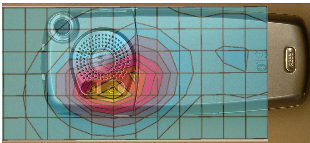
Figure 9. Typical 1900MHz W-CDMA Body Worn Contour Overlaid on Phone
