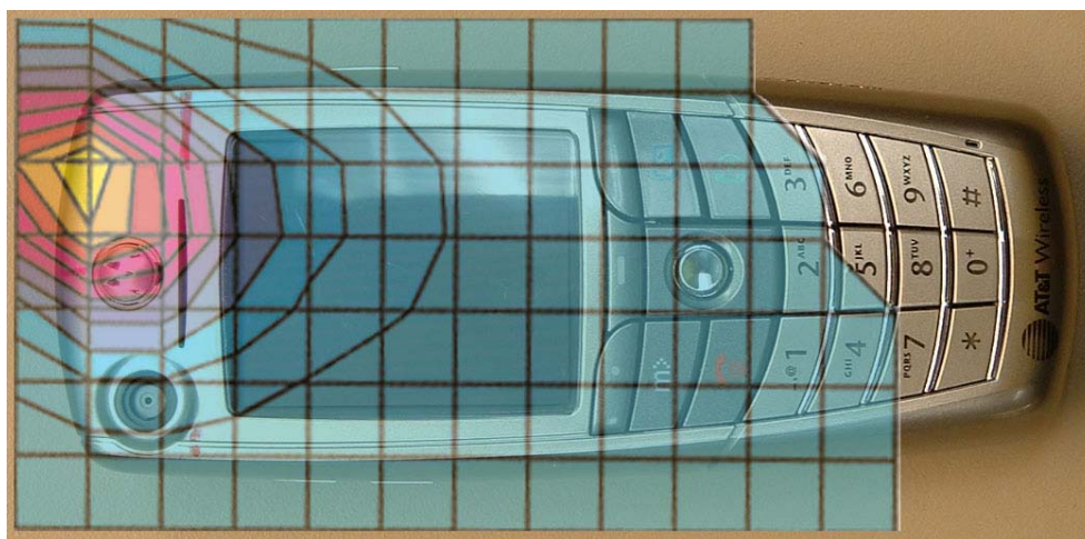
Figure 5. Typical 1900MHz GSM Head Adjacent Contour Overlaid on Phone (15 ° Tilt)
