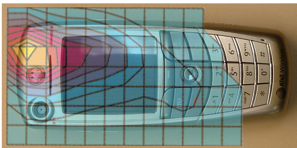
Figure 3. Typical 1900MHz W-CDMA Head Adjacent Contour Overlaid on Phone (Cheek Touch)
