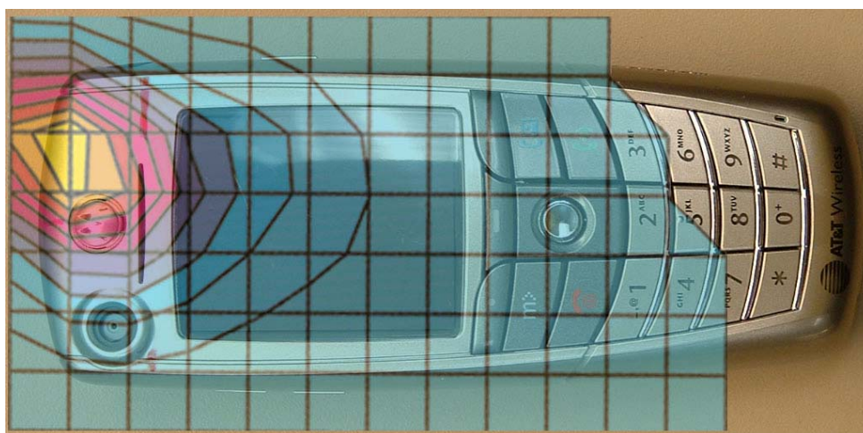
Figure 6. Typical 1900MHz W-CDMA Head Adjacent Contour Overlaid on Phone (15 ° Tilt)
