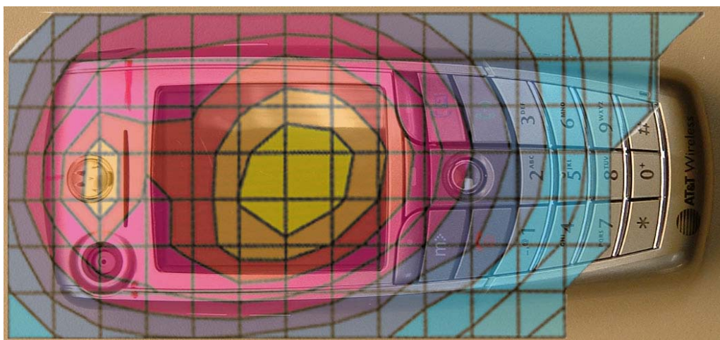
Figure 4. Typical 850MHz GSM Head Adjacent Contour Overlaid on Phone (15 ° Tilt)
