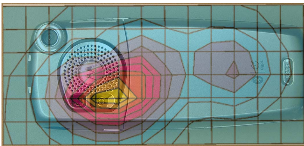
Figure 8. Typical 1900MHz GSM Body Worn Contour Overlaid on Phone
