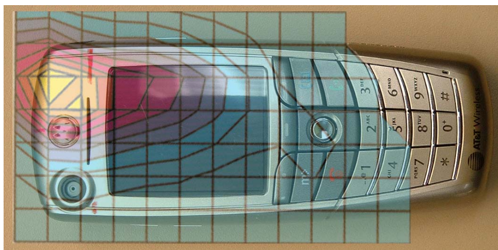
Figure 2. Typical 1900MHz GSM Head Adjacent Contour Overlaid on Phone (Cheek Touch)
