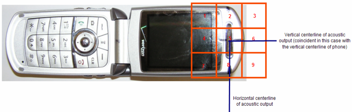
Figure A2-3. Phone Open – 5cm x 5cm grid for Near Field Measurements
