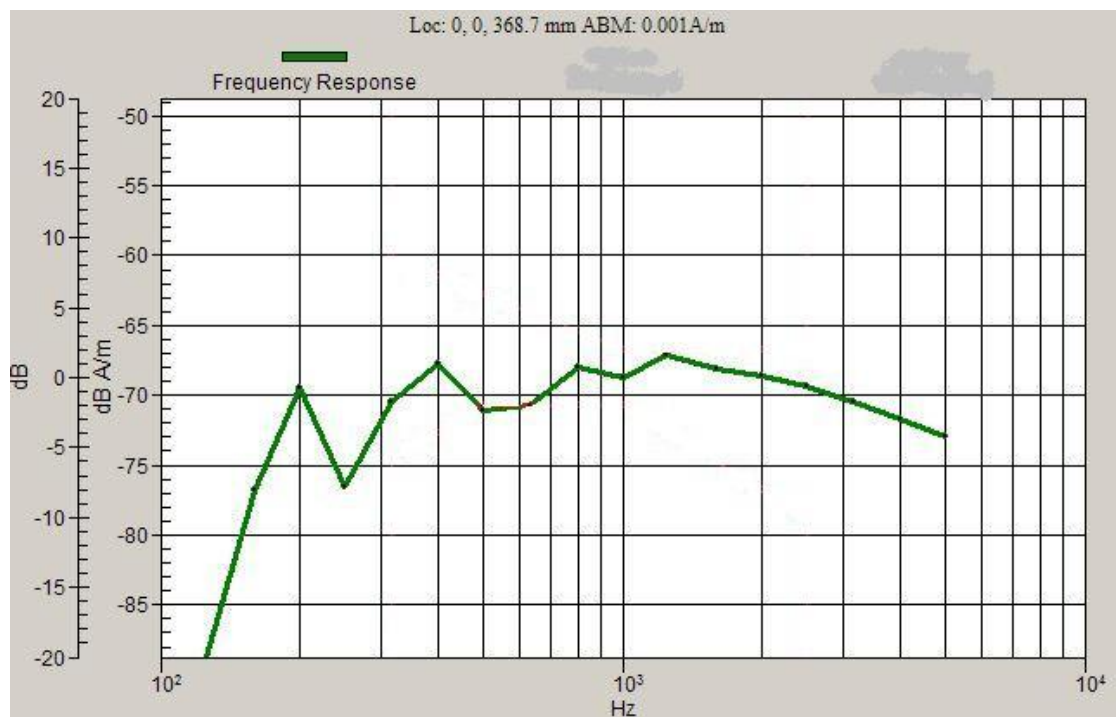
Graph A1-2. Radial 1 Position Ambient Noise Spectrum Plot
