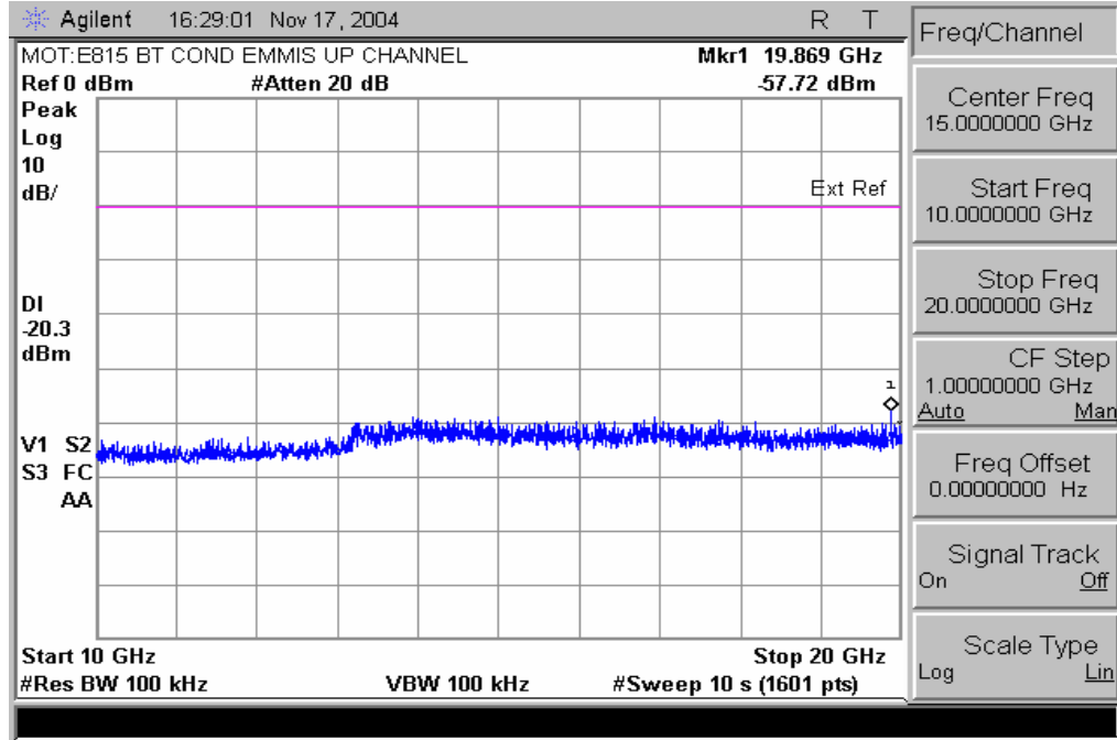
Conducted Spurious Emissions 10-20GHz (High Channel Enabled)
