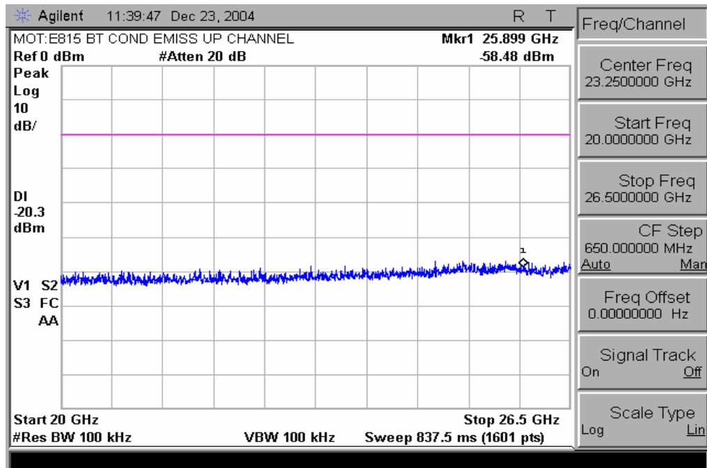
Conducted Spurious Emissions 20-26.5GHz (High Chan Enabled)
