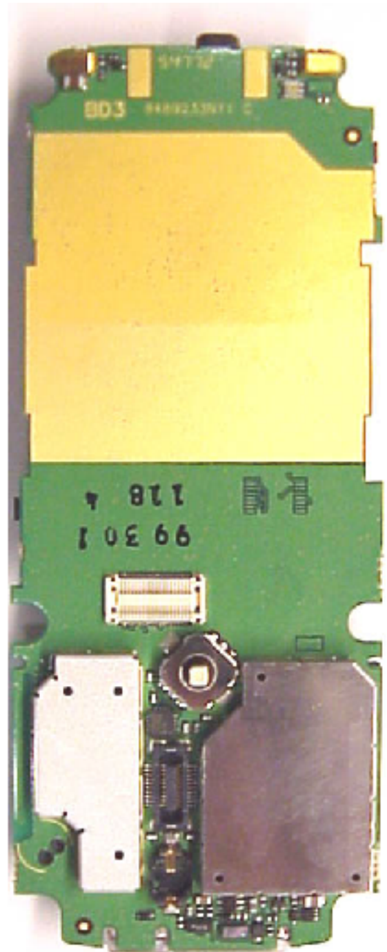
Front View with Shields
