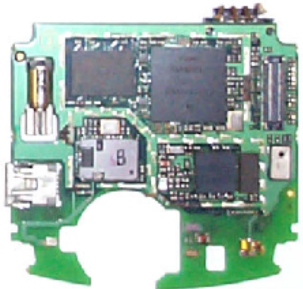
Rear View (Shields Removed)
