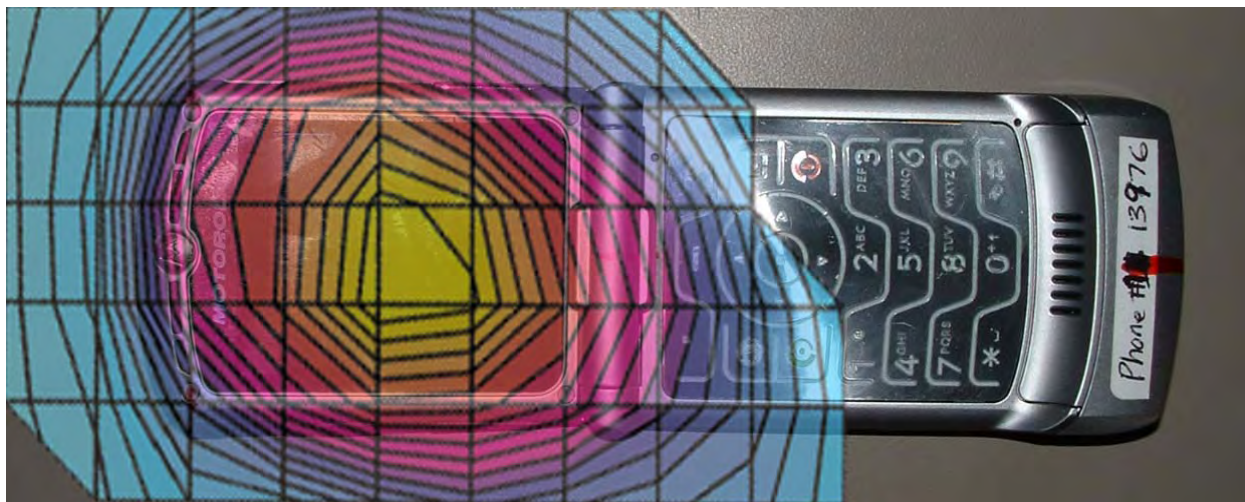
Figure 3. Typical 850MHz GSM Head Adjacent Contour Overlaid on Phone (15 ° Tilt)
