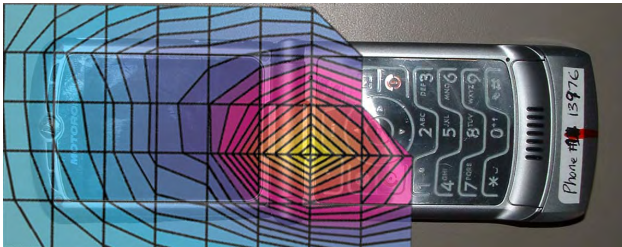
Figure 1. Typical 850MHz GSM Head Adjacent Contour Overlaid on Phone (Cheek Touch)
