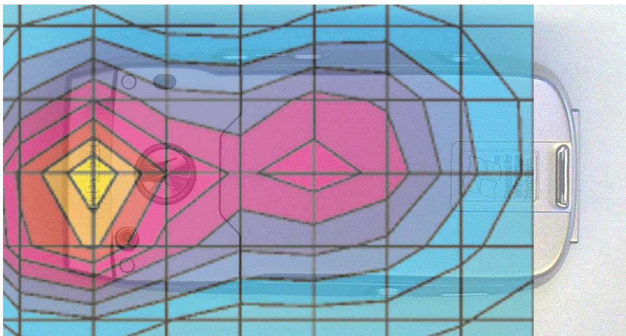
Figure 6. Typical 1900 MHz Body-Worn Contour Overlaid on Phone
