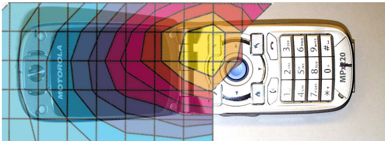
Figure 3. Typical 850MHz Head Adjacent Contour Overlaid on Phone (15 ° Tilt)
