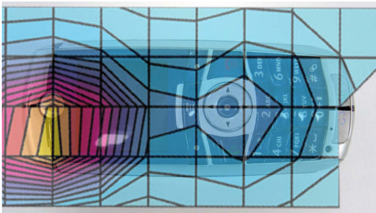
Figure 4. Typical 1900MHz GSM Head Adjacent Contour Overlaid on Phone (15 ° Tilt)
