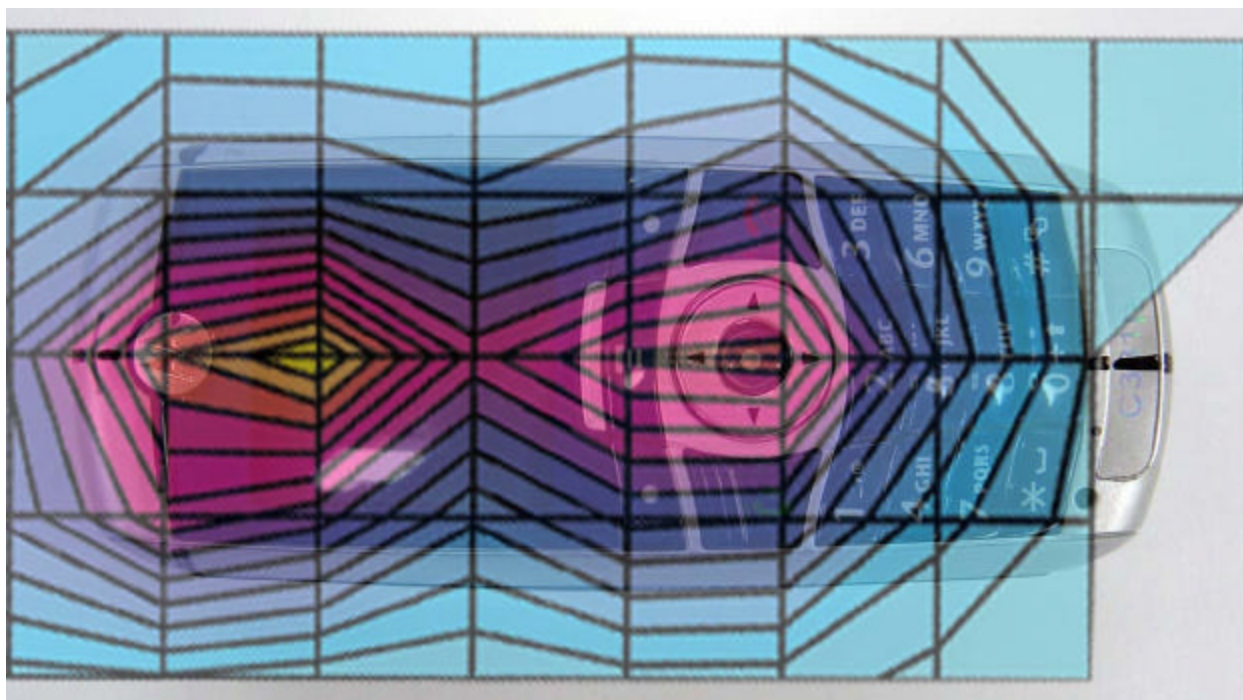
Figure 2. Typical 1900MHz GSM Head Adjacent Contour Overlaid on Phone (Cheek Touch)
