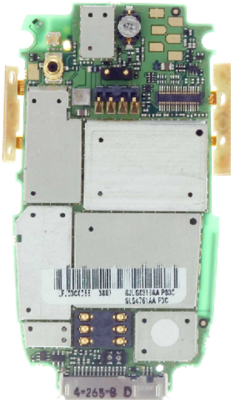
Rear Views
