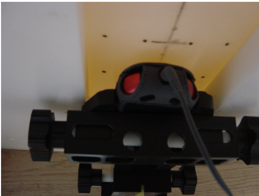
Figure 4. Phone with Arm Band Case SYN1697A Against the Flat Phantom
