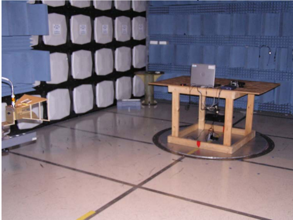
Radiated Emissions Measurement Setup
