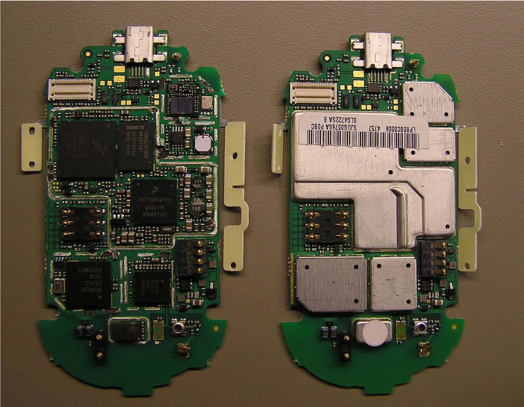
MAIN BOARD W/O SHIELDS
