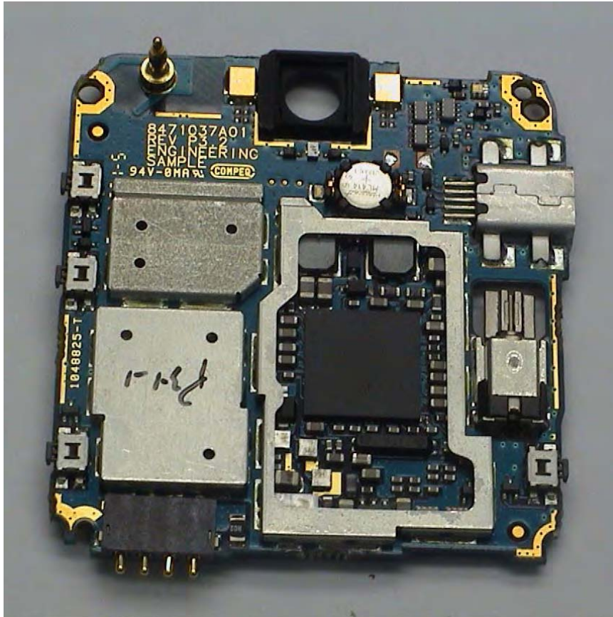
Rear View With Shields Removed
