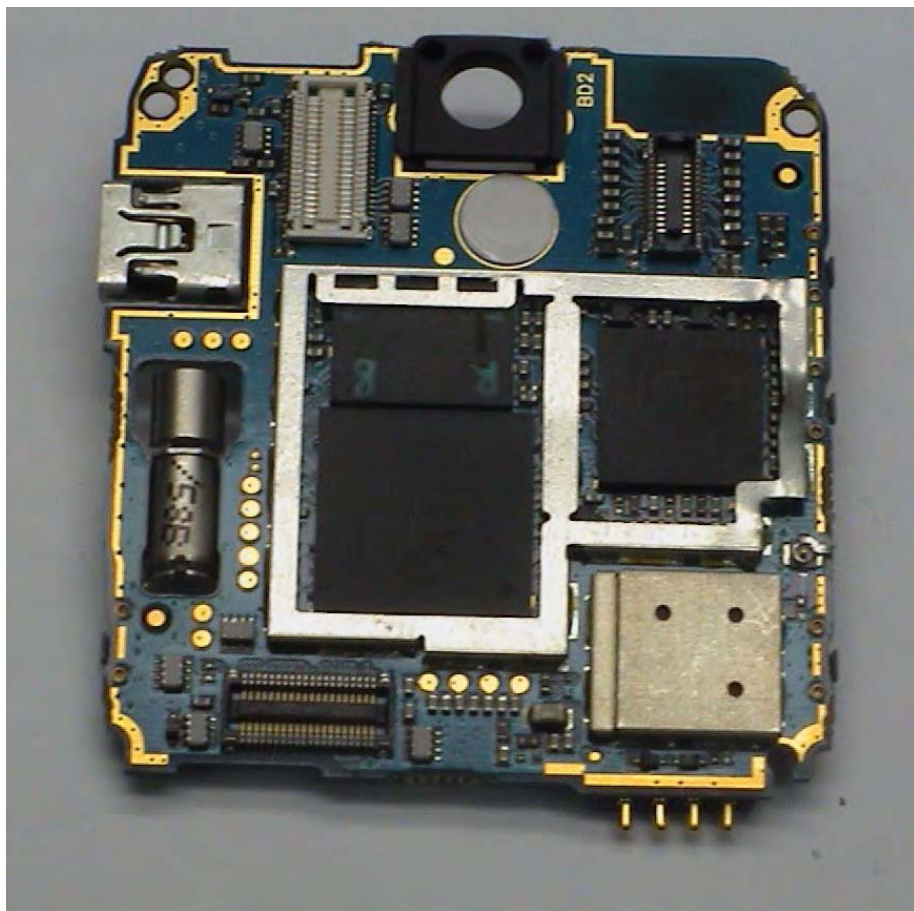
Front View With Shields Removed
