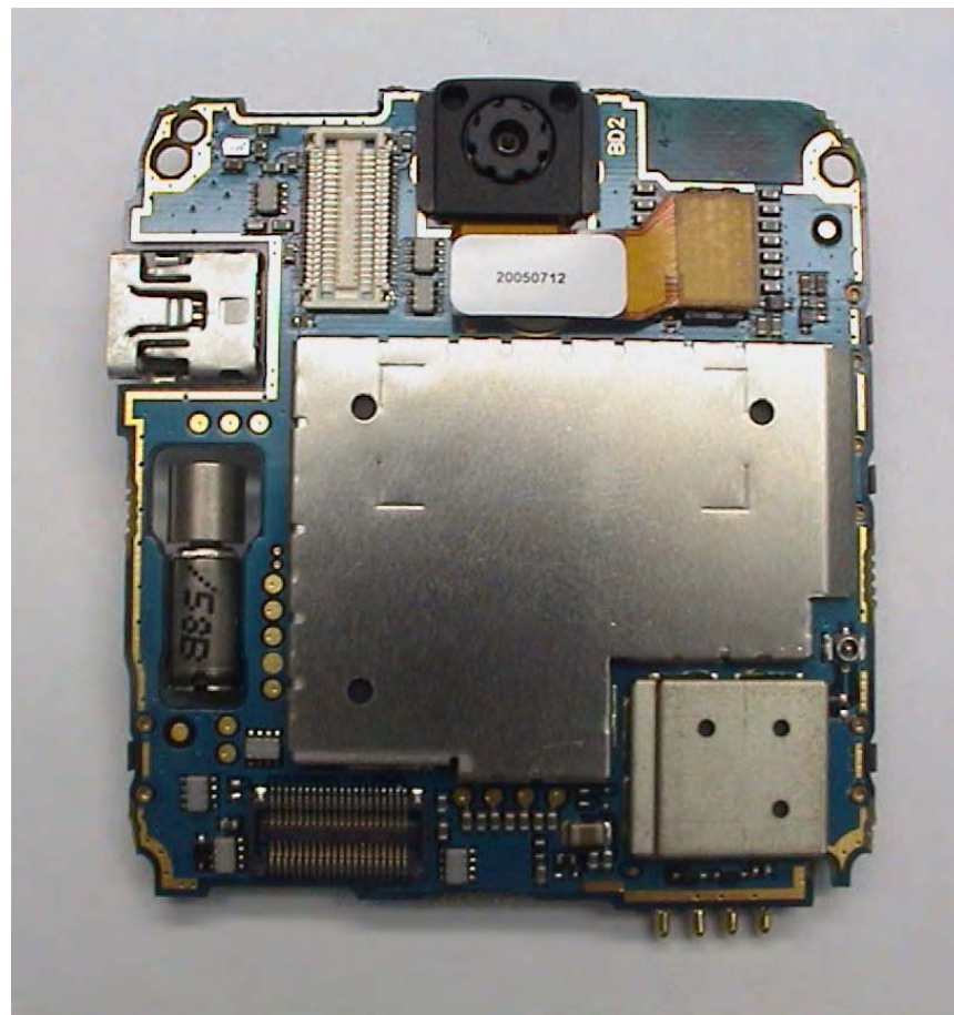
Main PCBA (Front View)
